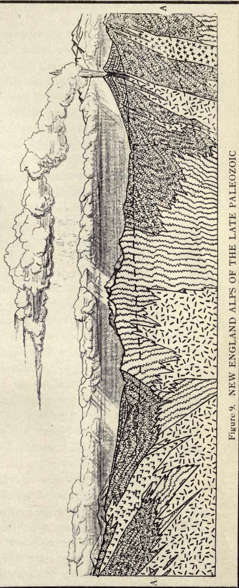
Figure 8. BEGINNING OF THE TRIASSIC SEDIMENTATION
