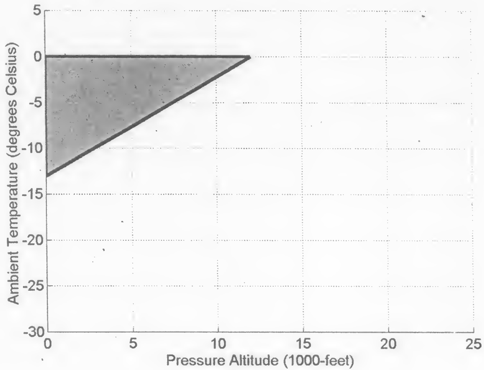
FIGURE 6 - Appendix O, Freezing Rain, Temperature and Altitude
