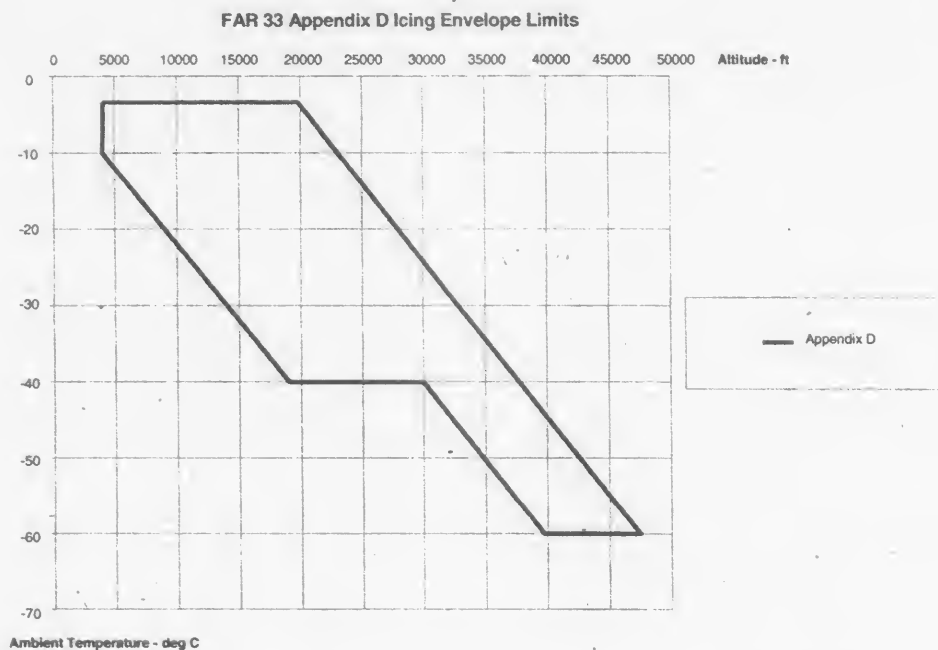
Figure D1 - Convective Cloud Ice Crystal Envelope
