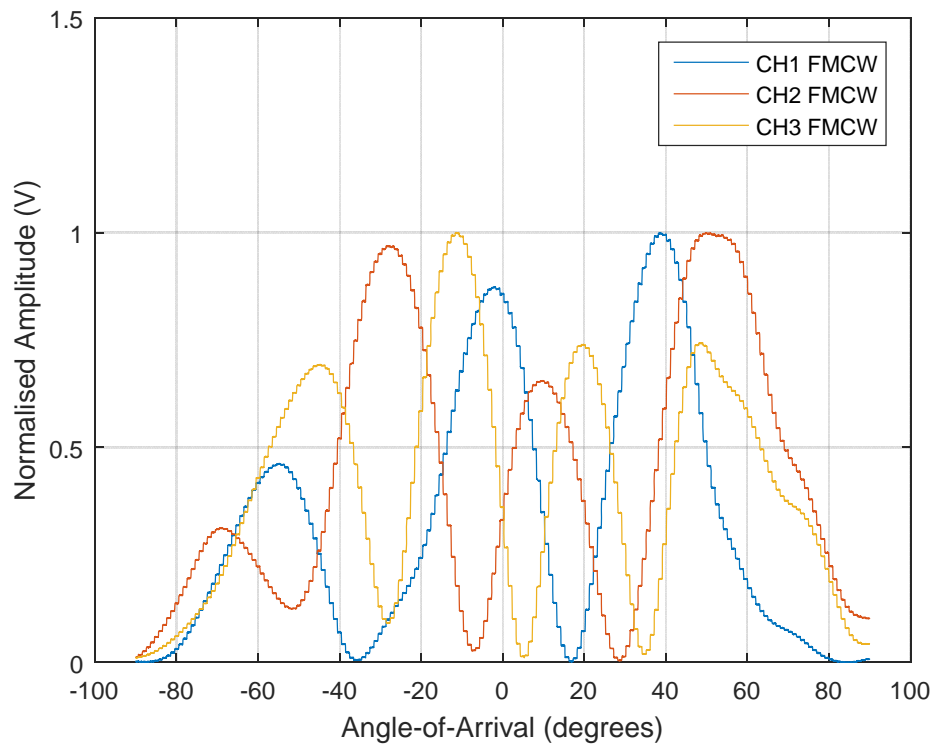
Figure 46. FMCW Data after Post-processing and Normalization (July 13, 2016)
