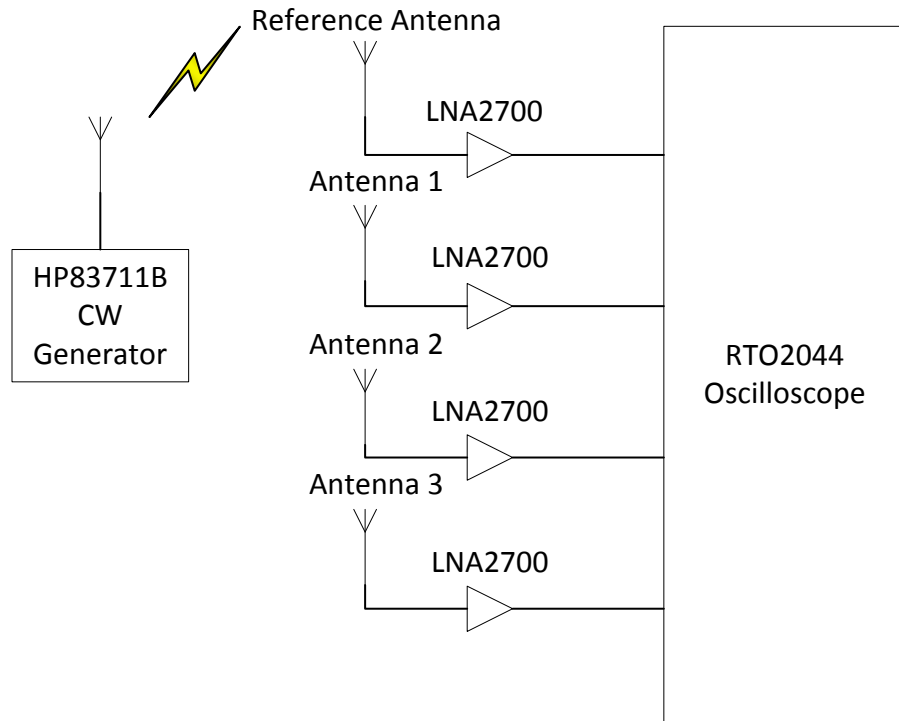
Figure 12. Calibration Setup for Front-end Antenna Sub-system
