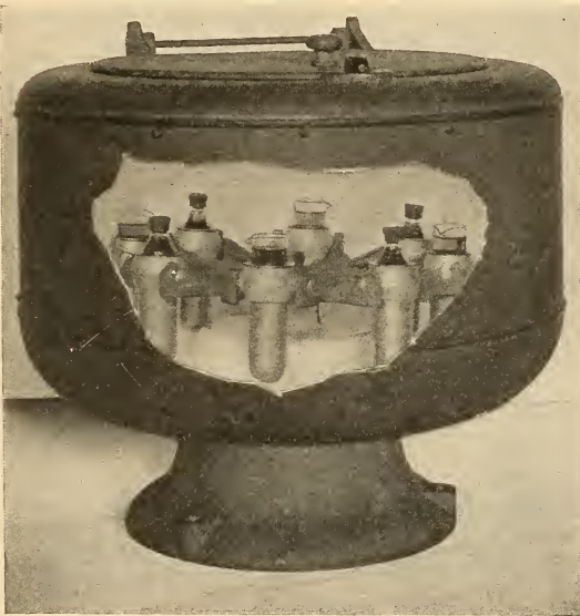
FIG. 121.—Centrifuge, size 1, type B, with 8-tube, 50 c.c. head, manufactured by the International Instrument Co.
