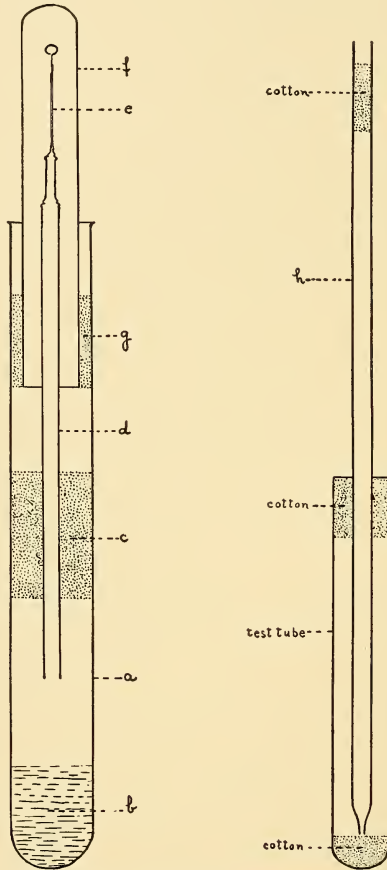
FIG. 18.—McJunkin's tube for collecting blood for cultures.
