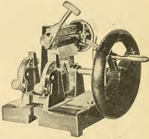
FIG. 120.—Minot rotary microtome (International Instrument Co., Cambridge, Mass.).
