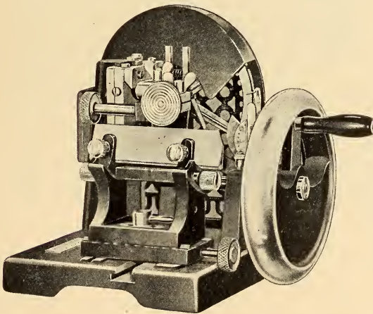
FIG. 119.—Minot's wheel microtome (Bausch & Lomb).
