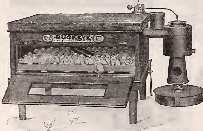
Buckeye No. 14, Style E, 65-Egg Incubator
