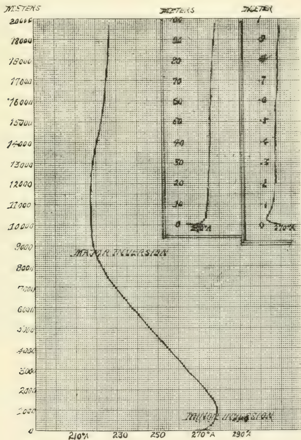
FIG. 1. TEMPERATURE INVERSIONS.
