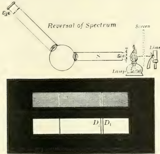
FIG. 12. THE SPECTROSCOPE.
