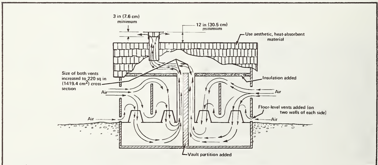
Figure 10. Good multi-hole venting design minimizes bad odors.
