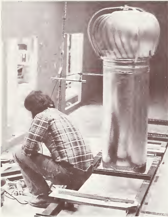
Figure 5. Turbine ventilator test setup.
