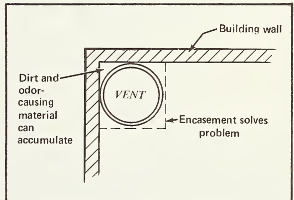
Figure 8. Round vent in square corner.
