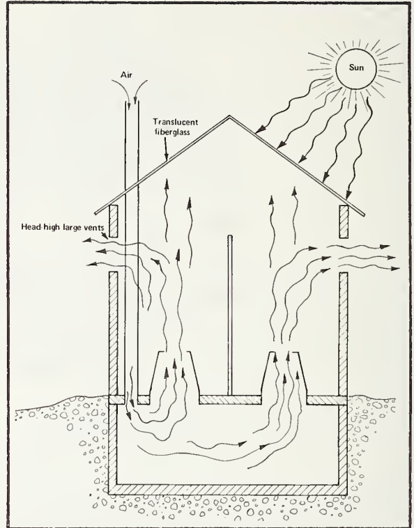
Figure 14. Poor roof design concentrates odors.
