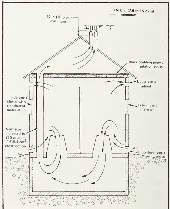
Figure 15. Good roof design minimizes odors.
