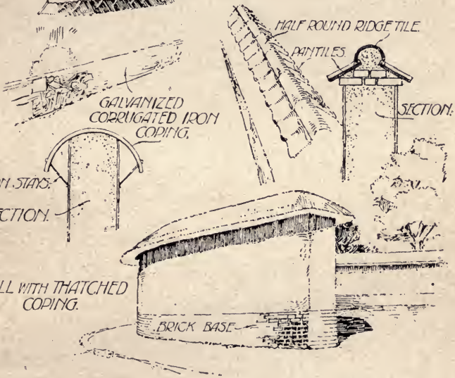
DETAILS OF CHALK CONSTRUCTION AT AMESBURY.
