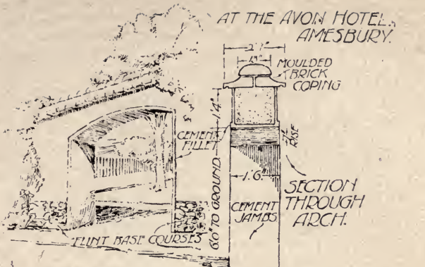
DETAILS OF CHALK CONSTRUCTION AT AMESBURY. TILE AND BRICK COPING.
