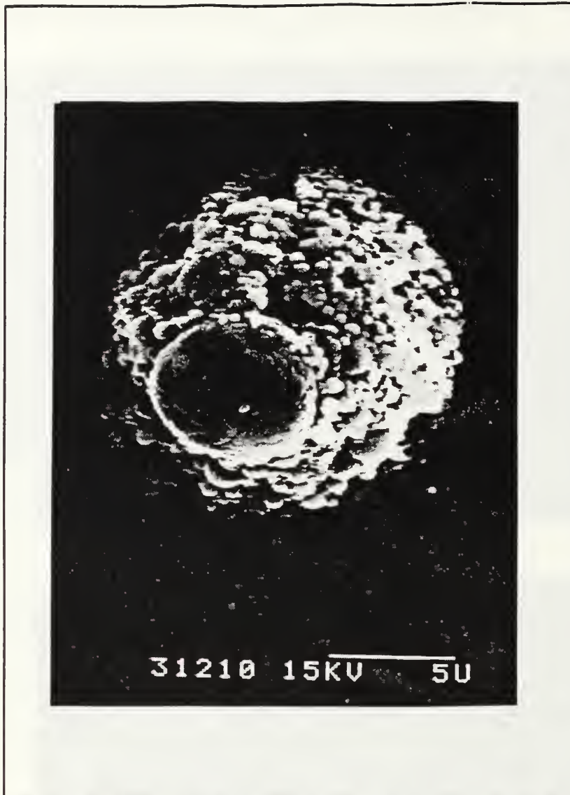
Figure 4.4. Example of Large Agglomerate from Test 3-12.
