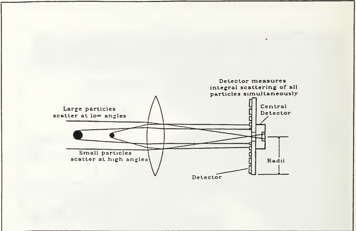
Figure 2.2. Malvern Light Scattering Principle [Ref. 11, p. 1-16].
