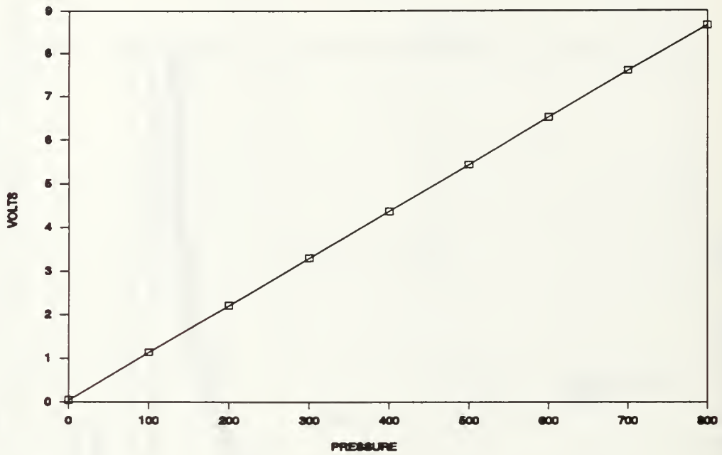
Figure 3.1. Pressure Calibration of Transducer During Pre-fire Check.
