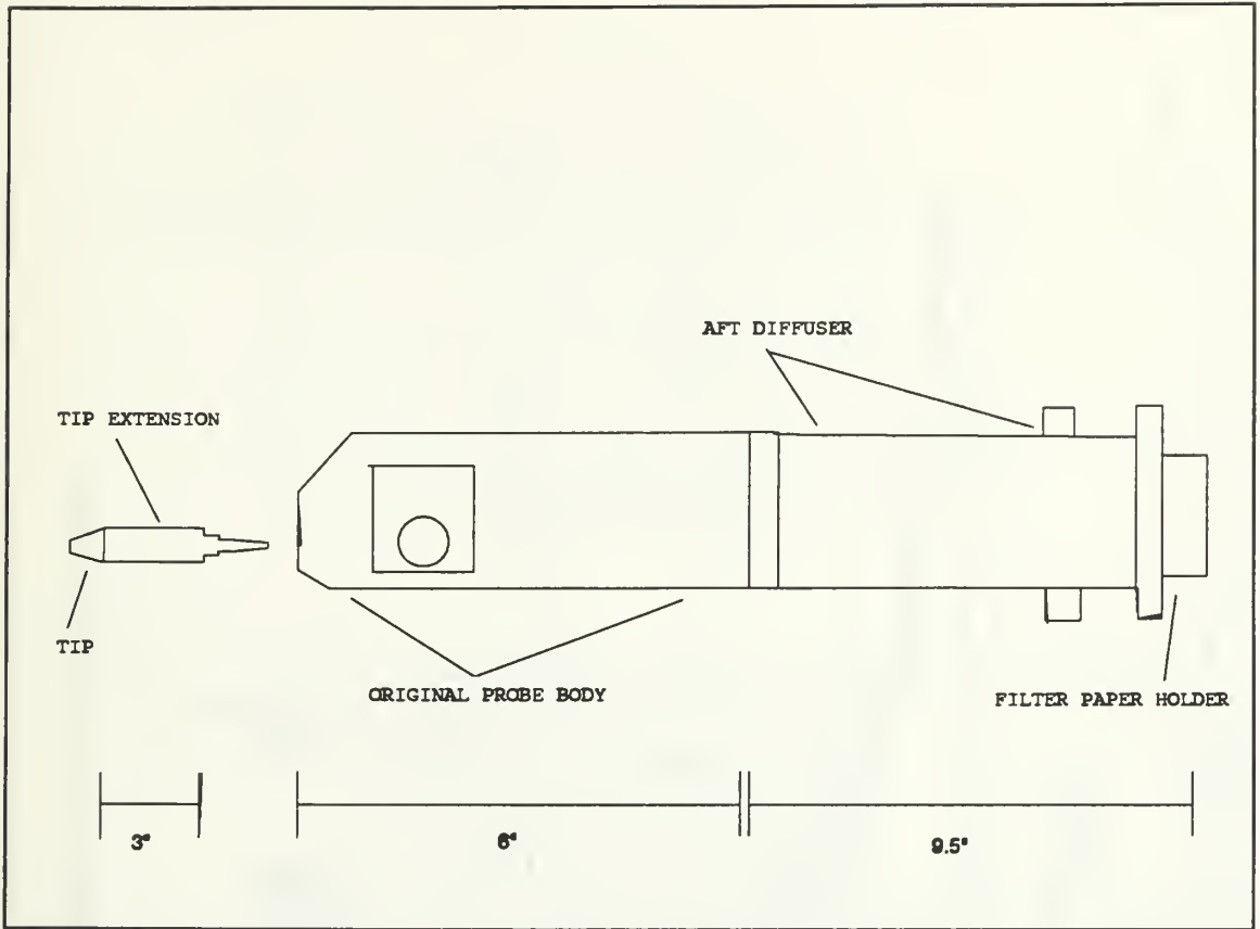
Figure 2.5. Probe After Modification.
