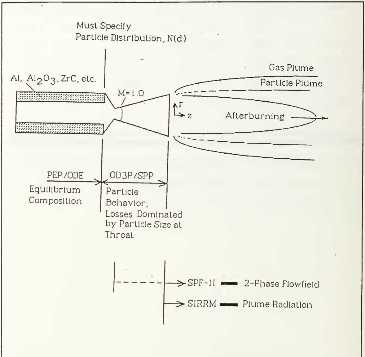
Figure 1.1. Sequence of Computer Codes in the Calculation of Rocket Motor Performance and Plume Signature.
