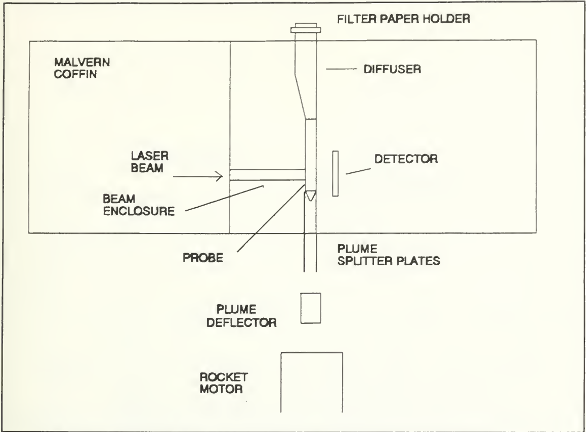
Figure 2.3. Malvern Enclosure and Plume Splitter.
