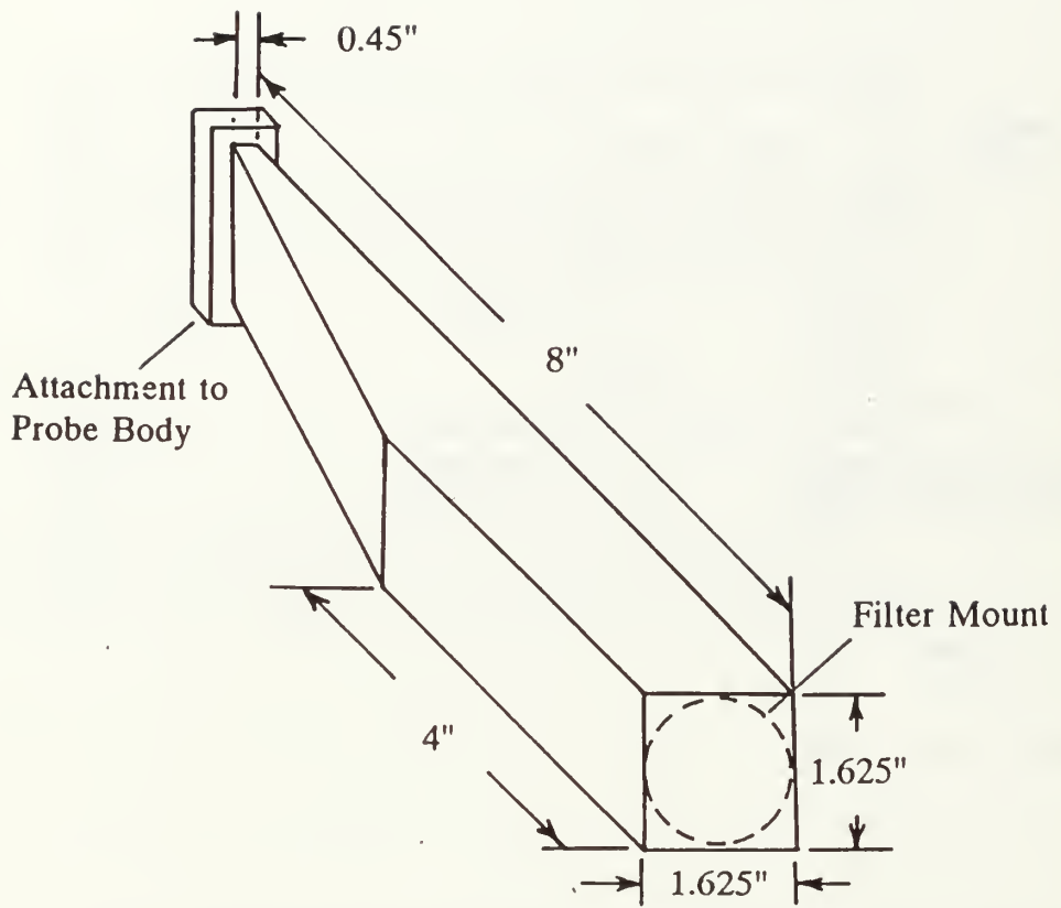
COLLECTION PROBE EXTENSION/DIFFUSER
