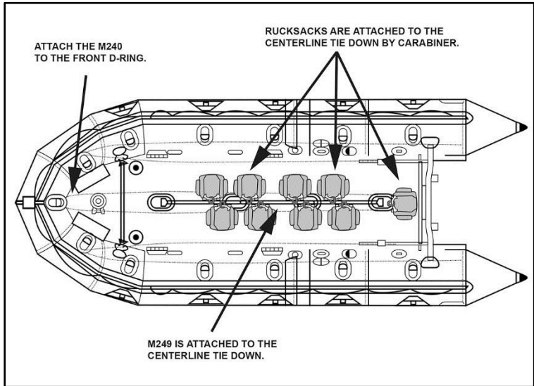
Figure 12-5. Equipment rigging
