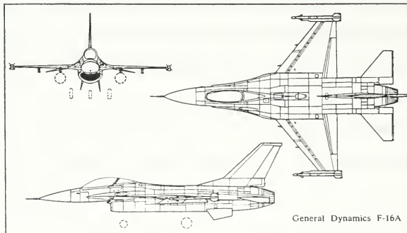
Figure 34. F-16 General Arrangement. From Ref. [20].
