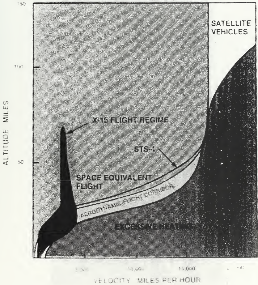
Figure 18. X-15 Flight Regime. From Ref. [9].
