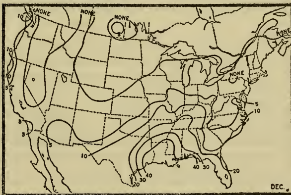
FIGURE 10.—Monthly isokeraunic maps based upon the total number of thunderstorm days occurring each month over the 20-year period 1904-23. Divide the numbers on the maps by 20 to obtain the average number of thunderstorm days to be expected per month. (After Alexander.)
