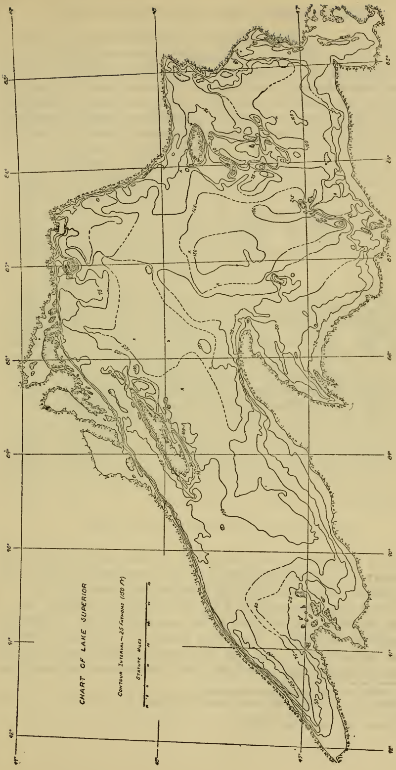
FIGURE 5.—Contour map of Lake Superior. Depths in fathoms.
