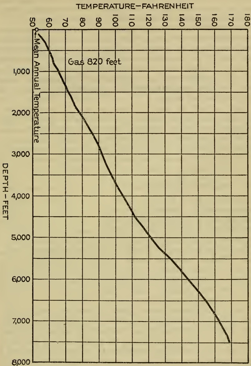
FIGURE 3.—Curve showing the temperatures of the rocks for various depths, increasing, but increasing more rapidly at the bottom, indicating a heat wave which has not reached the bottom. (C. E. Van Orstrand, On the nature of isogeothermal surfaces, Amer. Journ. Sci., vol. 15, p. 514, fig. 8, June 1928.)
