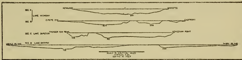
FIGURE 2.—Cross-sections of the Great Lakes. Note the relatively steep sides and broad base.
