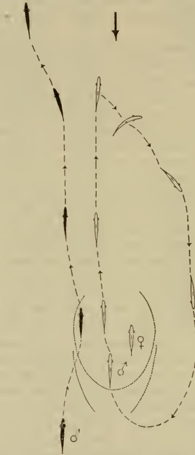
FIGURE 3.—A diagram illustrating the escorting act of the male redfish, Oncorhynchus nerka . Note that the female, ♀ (dotted) remains over the nest while the male, ♂, drives the invader (solid black) away. The male and female are shown in their positions over the nest. Drawn by Dan Merriman. Courtesy Mid-Pacific Magazine.
