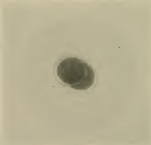
3. MICROPHOTOGRAPHS OF OVERLAPPING URANIUM HALOS.
