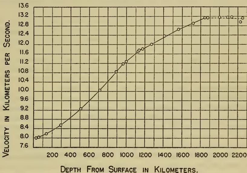
FIGURE 1.—Velocity-depth curve (after Repetti). Such curves supply direct evidence concerning the nature of the earth's interior.
