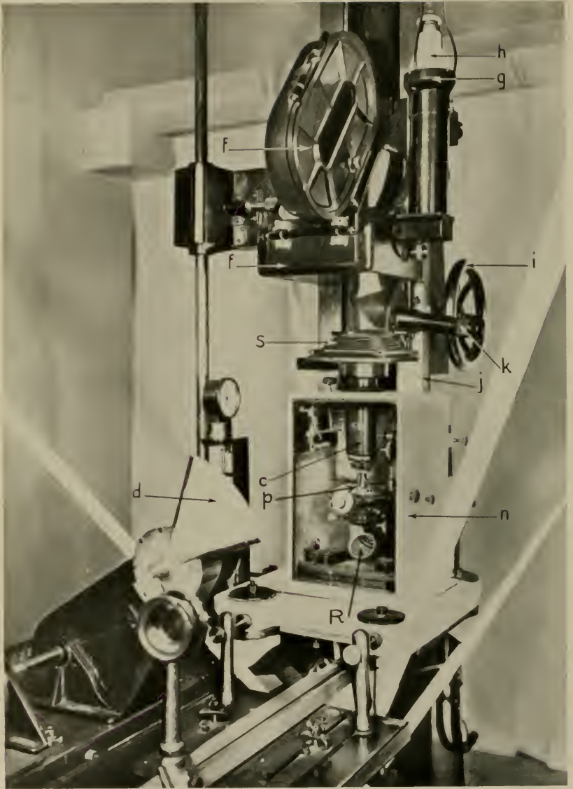
The microscope c placed in a controlled temperature chamber n .
