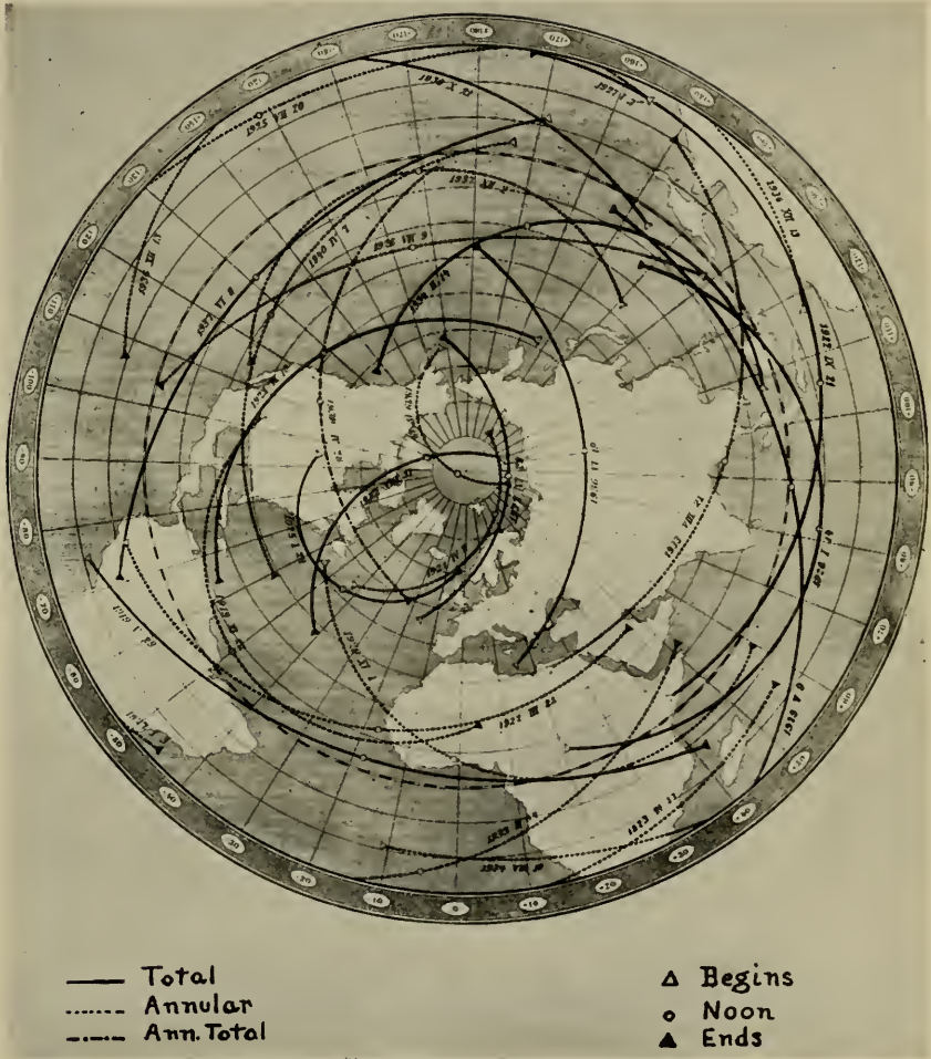
TRACKS OF SOLAR ECLIPSES BETWEEN THE YEARS 1919 AND 1940.
