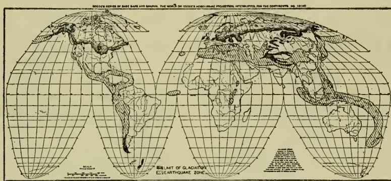
FIGURE 4.—Showing the lack of relation between earthquake belts and glaciated territory.
