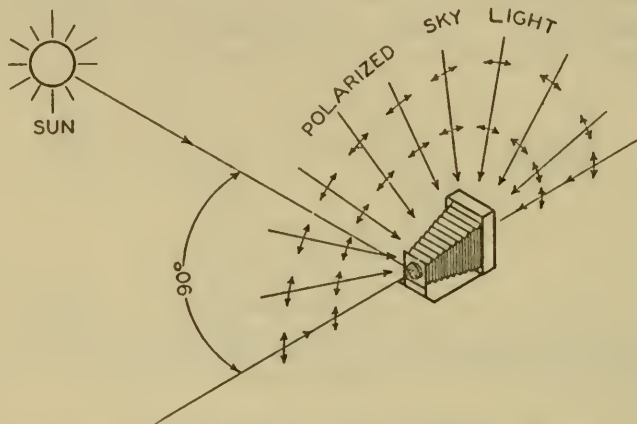
CLEAR BLUE SKYLIGHT ARRIVING AT RIGHT ANGLES TO THE SUN'S RAYS IS POLARIZED.
