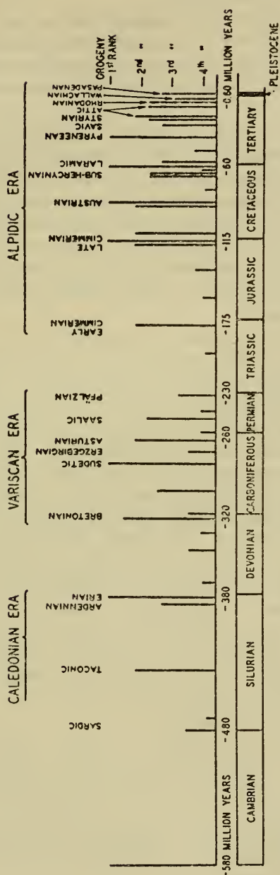
Figure 2.—Dates, by abscissas, and importance, of the mountain-building (orogenic) upheavals of the past. (After Stille.)
