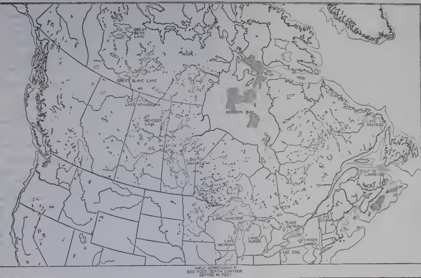
FIGURE 1.—Showing the basins associated with glaciation in North America. Depths are in feet. The principal basins on the continental shelves are shaded.
