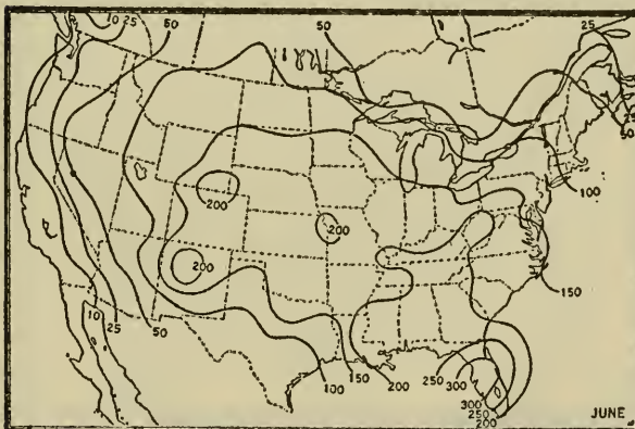
FIGURE 8.—Monthly isokeraunic maps based upon the total number of thunderstorm days occurring each month over the 20-year period 1904-23. Divide the numbers on the maps by 20 to obtain the average number of thunderstorm days to be expected per month. (After Alexander.)
