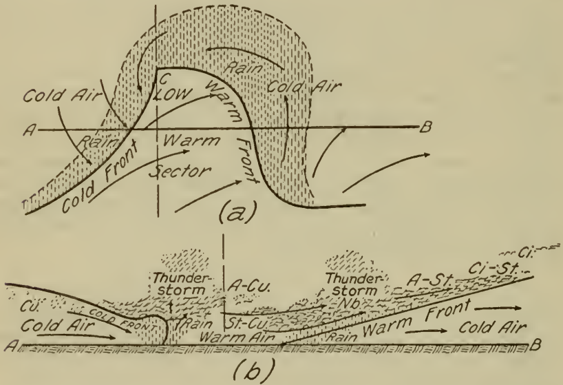
FIGURE 5.—Horizontal (a) and vertical (b) cross-sections through a low-pressure system, showing the cold-front and the warm-front. Ci., Ci-St., etc., refer to types of cloud. (After Bjerknes and Solberg.)
