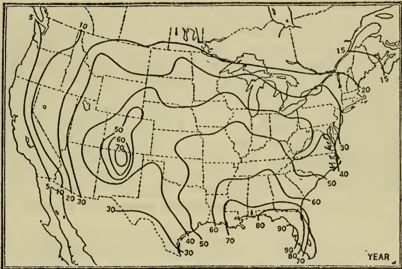
FIGURE 11.—Isokeraunic map indicating the average number of thunderstorm days to be expected per year throughout the United States; based on 20-year records covering the period from 1904 through 1923. (After Alexander.)
