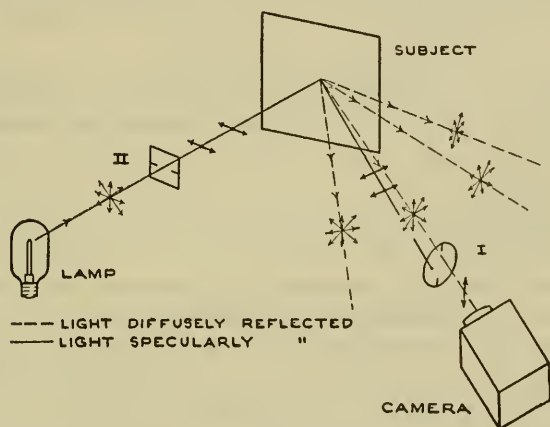
FIGURE 4.—Photography by diffusely reflected light, using Eastman Pola-screens. Light reflected specularly retains its polarized form; it may therefore be cut out by a Pola-screen at the camera. I indicates a Pola-screen, type I; II indicates a large Pola-screen, type II. The indexes on the two Pola-screens show their planes of vibration.
