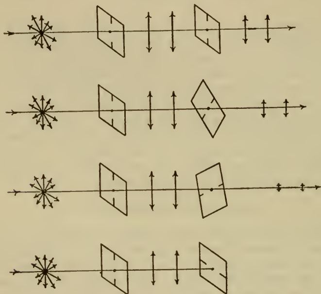
FIGURE 1.—Light rays are polarized by the Pola-screen at the left, the vibration plane of which is shown vertically. The amount of light let through by the second Pola-screen is cut down as the Pola-screen is turned. When the vibration plane of the second Pola-screen is at right angles to the first, practically no oblique light gets through.
