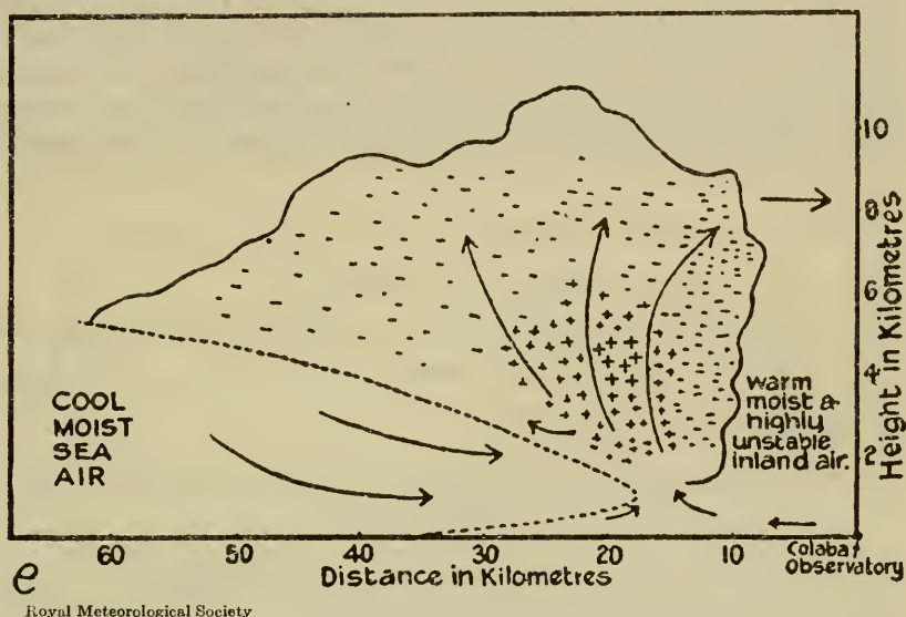
FIGURE 2.—Distribution of electrical charge in a thunderstorm. (After Banerji.)
