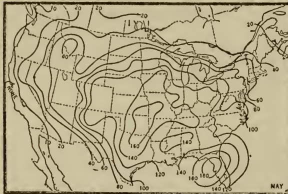
FIGURE 7.—Monthly isokeraunic maps based upon the total number of thunderstorm days occurring each month over the 20-year period 1904-23. Divide the numbers on the maps by 20 to obtain the average number of thunderstorm days to be expected per month. (After Alexander.)
