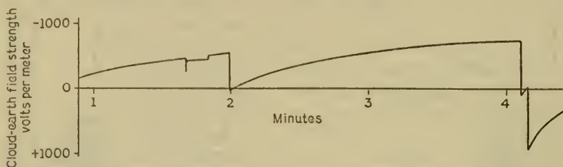
FIGURE 3.—Regeneration of the electrical field between a cloud and the earth after a lightning discharge. (After Wilson.)
