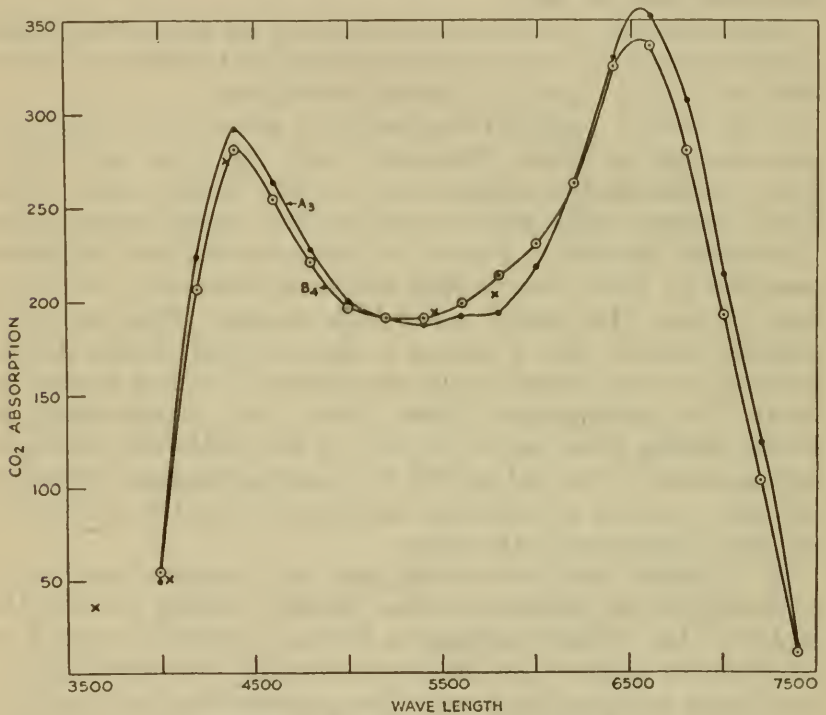
FIGURE 1.—Wave-length assimilation curves.
