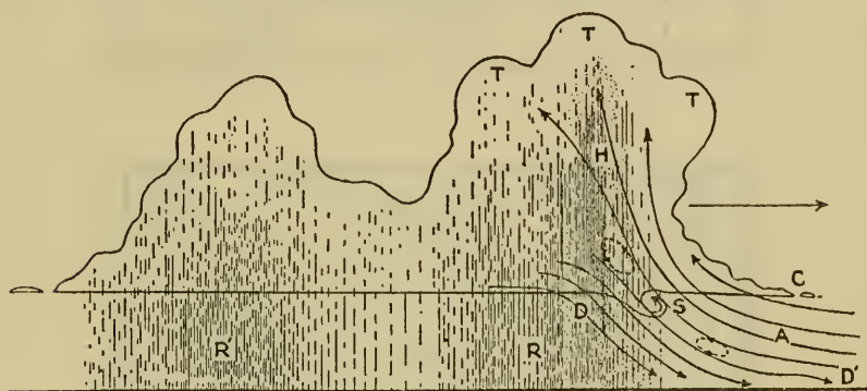
FIGURE 6.—Schematic cross-section of a thunderstorm showing adjacent downward and upward air currents which help maintain the storm. A , ascending air; D , descending air; C , storm collar; S , roll scud; D' , wind gust; H , hail; T , thunderheads; R , primary rain; R' , secondary rain. (After Humphreys.)
