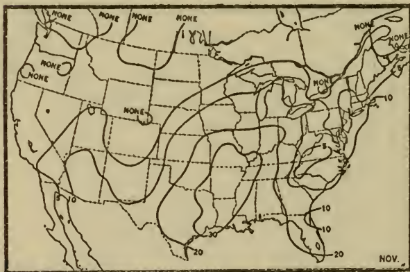
FIGURE 9.—Monthly isokeraunic maps based upon the total number of thunderstorm days occurring each month over the 20-year period 1904-23. Divide the numbers on the maps by 20 to obtain the average number of thunderstorm days to be expected per month. (After Alexander.)
