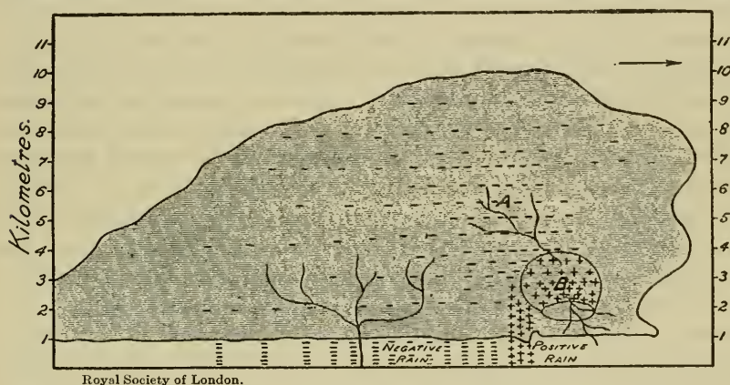
FIGURE 1.—Distribution of electrical charge in a heat thunderstorm. (After Simpson.)
