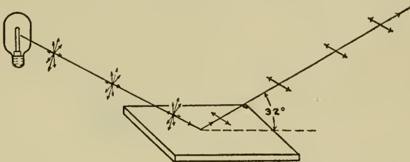
FIGURE 2.—Ray polarized by reflection. A ray of ordinary, unpolarized light is almost completely polarized when specularly reflected at about 32^\circ to any nonmetallic surface, such as glass. This permits subduing oblique reflections from glass and water by a single Pola-screen over the lens.
