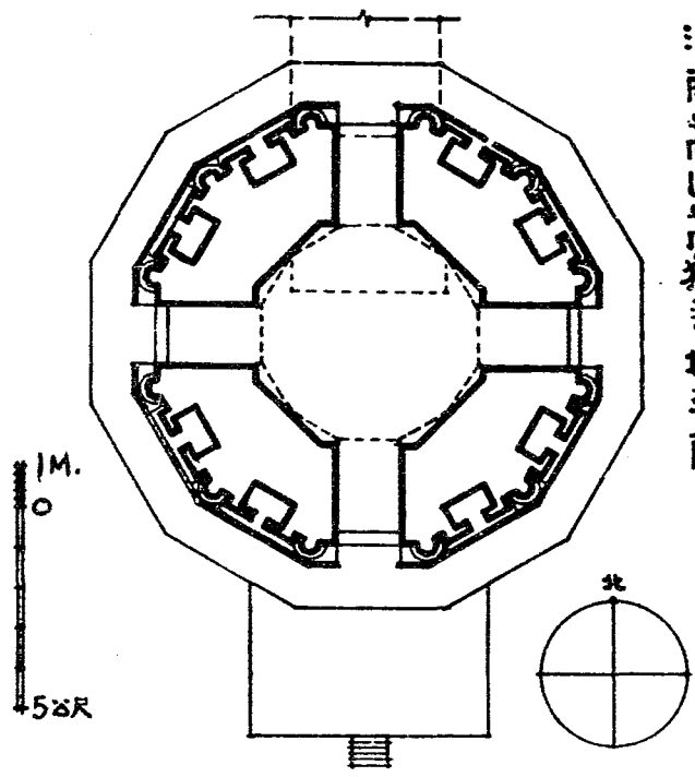
PLAN OF PAGODA, SONG-YÜEH SSÜ SONG-SHAN, HONAN
