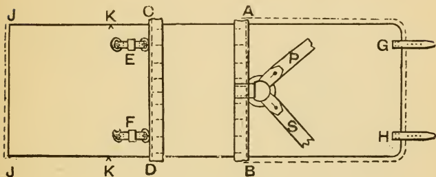
Fig. 100.—Body of Knapsack.
