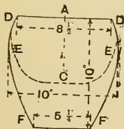
Fig. 71.—Gusset Pattern.
