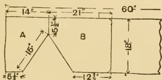
Fig. 141.—Pattern for Cycle Valise.
