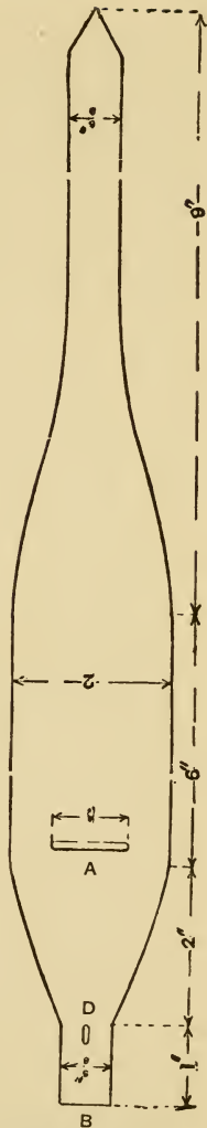
Fig. 14.—Pattern for Wrist Strap.
