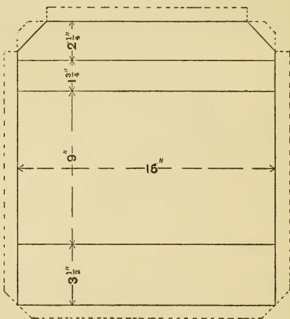
Fig. 133.—Pattern for Music Carrier.
