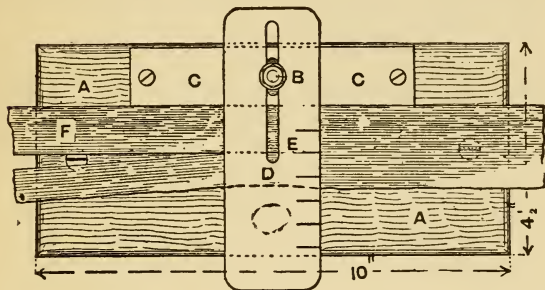
Fig. 20.—Strap Cutting Appliance.
