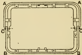
Fig. 69.—Brief Bag Frame.
