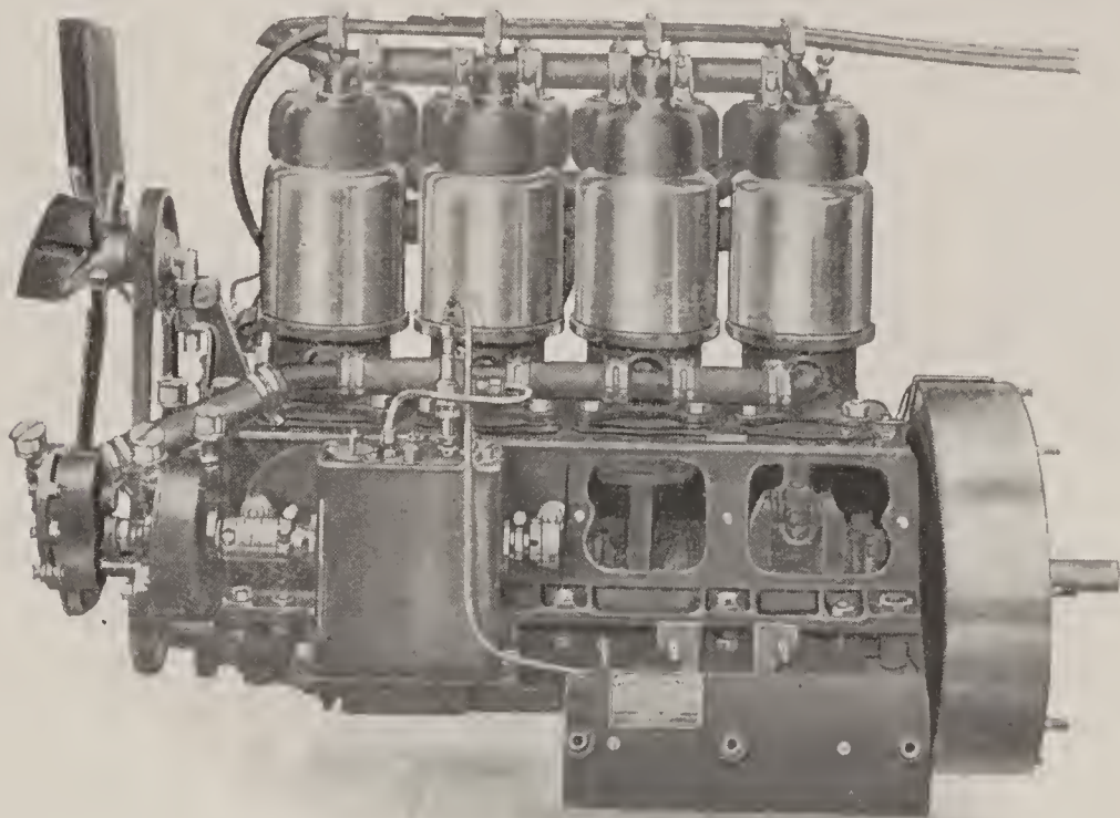
Fig. 13. Left Side of Cadillac 30-horsepower Engine
