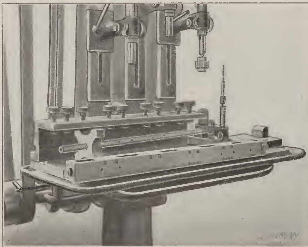
Fig. 24. Fixtures for Drilling and Reaming Cam-shafts
