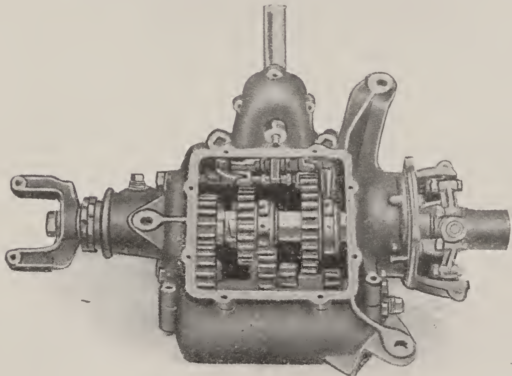
Fig. 18. Selective Type Sliding Gear Transmission
