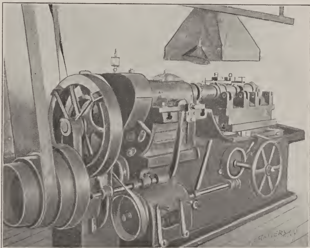
Fig. 25. Boring Cylinders
