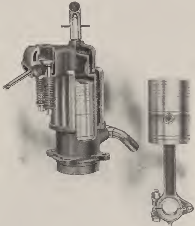
Fig. 17. The Cylinder and Piston
