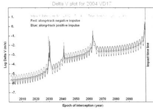
Fig. 2 The delta V plot developed by Carusi, Milani, et al. showing the change in velocity required to deflect asteroid 144898 2004VD17 from an Earth impact in 2102. This plot was incorporated into White Paper # 39 presented at NASA's 2006 NEO Workshop in Vail, Colorado to illustrate and emphasize the role of close gravitational encounters in shaping NEO deflections. The three discontinuities in this plot each represent a close pass of the NEO by the Earth in the decades prior to its potential impact with Earth in 2102.
