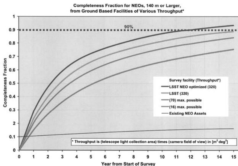
Figure 2. The completeness of several NEO surveys, based on LSST baseline cadence on the sky, is shown vs time from the start of the survey. The top two curves, with 15% and 5%, correspond to the LSST special NEO-optimized and the baseline LSST plan. The other curves represent the maximum possible completeness for less capable systems with smaller throughput. The top curve, based on 15% of the observing time spent in an NEO optimized mode, reaches the Congressional goal of 90% completeness for NEOs larger than 140m after 12 years of surveying. Given the timeline for agency approval of construction funding, it is likely that the LSST will have first light in 2014 and the sky survey will begin in 2015. With the survey start in 2015, the completeness for 140m and larger objects achieved in 2020 would be 70%, with 90% completeness for 350m and larger objects. Facilities with throughput smaller than LSST's 320 square meters square degrees have corresponding less completeness as shown in the lower curves.
