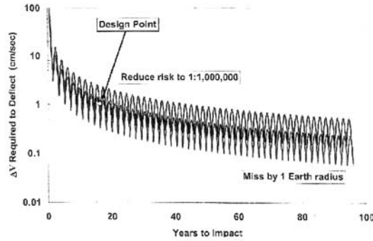
Figure 47. ΔV Required to Deflect Asteroid VD17 Fig. 3 The comparable plot from NASA's 2006 Near Earth Object Survey and Deflection Study showing the absence of close gravitational encounters prior to impact and the resultant factor of 1000 higher delta V required for deflection as a result of this omission.
