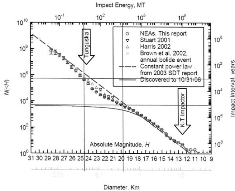
Figure 1. Size-frequency diagram for near-Earth objects, courtesy Alan Harris. The superposed intersecting lines bound the 99% of NEO impacts most likely to be encountered and trigger a call for deflection. These NEOs range from 45 – 400 meters in diameter. The left vertical line reflects the most recent estimate of the impact energy (5 MT) associated with the Tunguska event in 1908.
