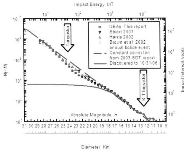
Fig. 1 The current size-frequency plot for near-Earth objects, presented at the March 2007 AIAA Planetary Defense Conference in Washington, DC by Alan W. Harris. This is an updated version of Fig. 2-3 from the 2003 NEO SDT study published by NASA in August 2003. For the purposes of this critique the differences between the 2003 and 2007 versions of this plot are insignificant.
