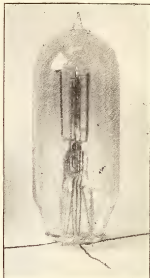
FIG. 10 After the tube has been exhausted and the glass stem sealed off, it resembles the completed tube except that it has no base
