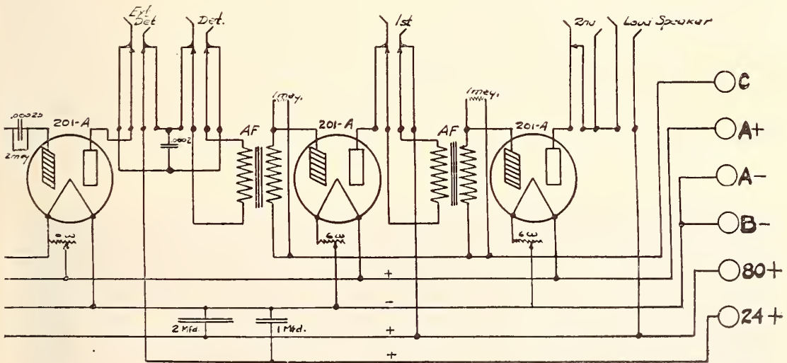
—AUDIO-FREQUENCY CIRCUITS
