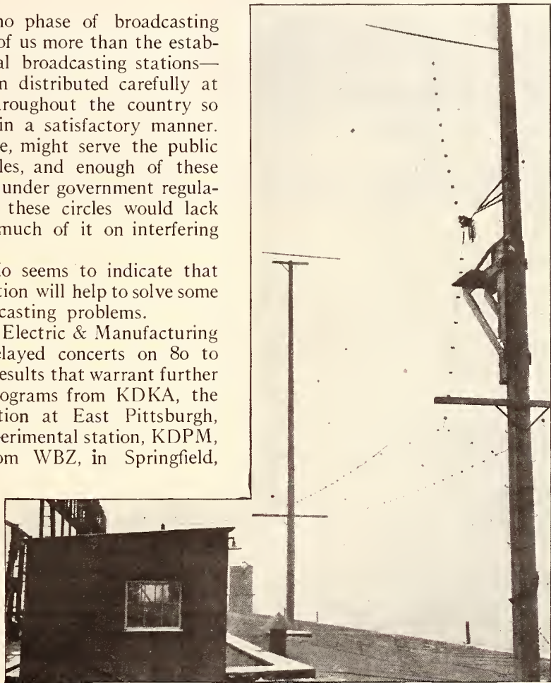
THE SHORT ANTENNA USED FOR 100-METER TRANSMISSION Erected at KDKA, East Pittsburgh, Pa.
