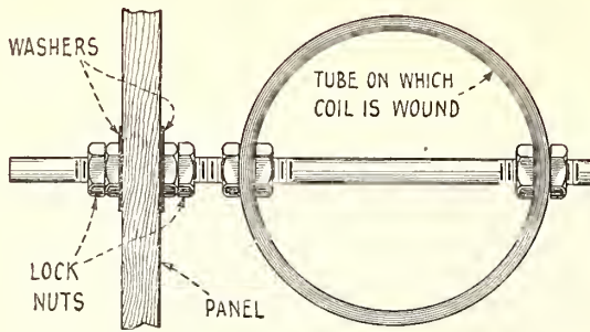
FIG. 2 Showing bearing for movable coils
