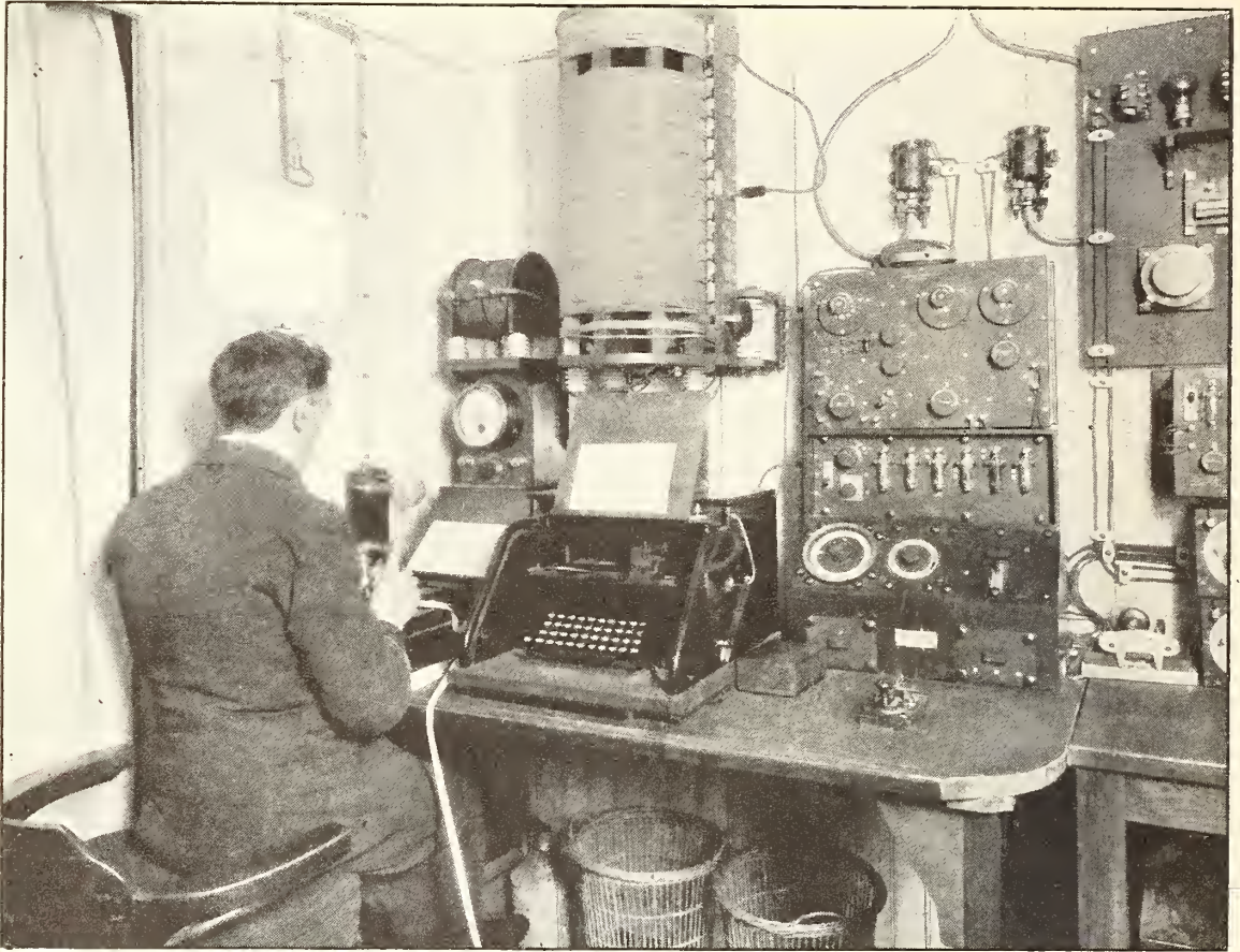
PREPARING MESSAGES TO BE SENT AT 80 WORDS A MINUTE
