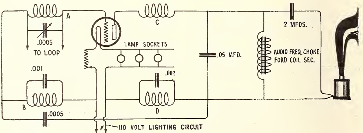
THE CIRCUIT ARRANGEMENT FOR THE ONE-TUBE LOUD SPEAKER LOOP RECEIVER
