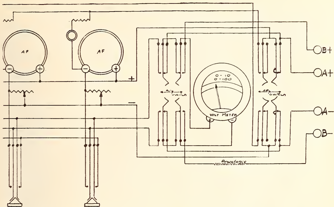
—CIRCUITS AS USED BY MR. BOSCOW IN HIS ELABORATE RECEIVER
