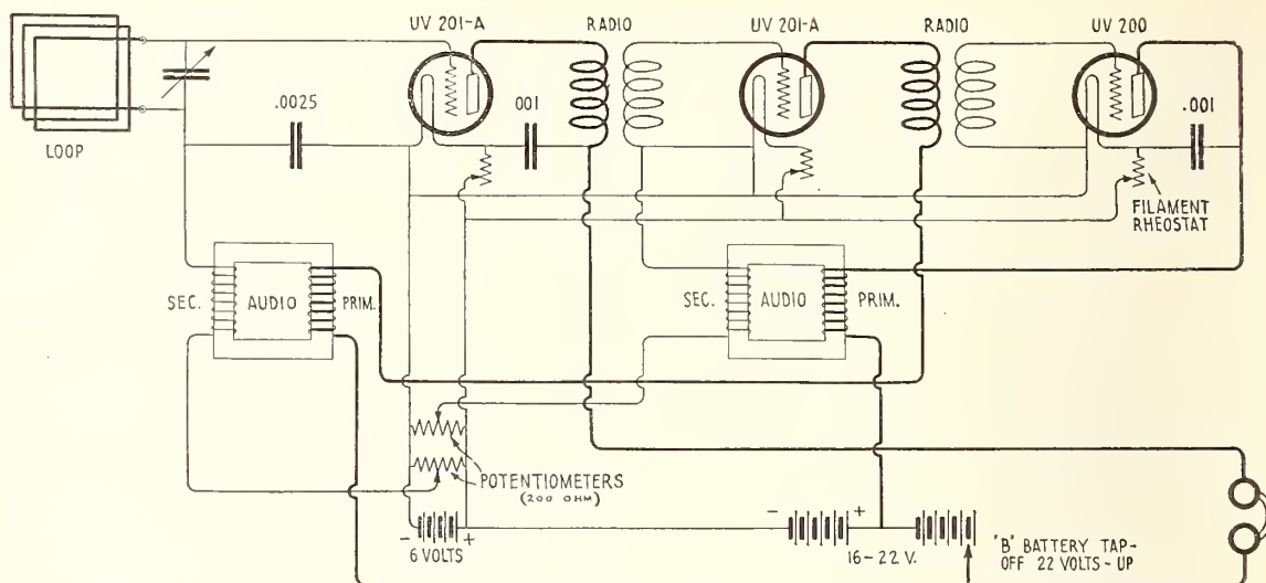
FIG. 5. THE STABILITY OF THE CIRCUIT IS IMPROVED BY TWO 200-OHM POTENTIOMETERS
