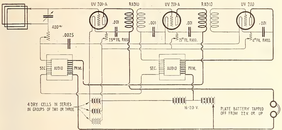
FIG. 1. HOW TO EMPLOY A UV-200 AND TWO 201-A'S
