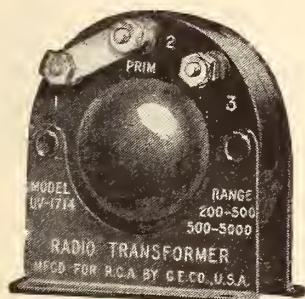
Model UV-1714 $6.50
