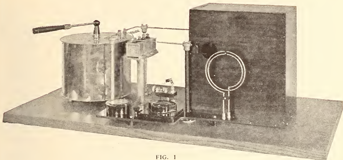
FIG. 1 Standard wavemeter of the Bureau of Standards
