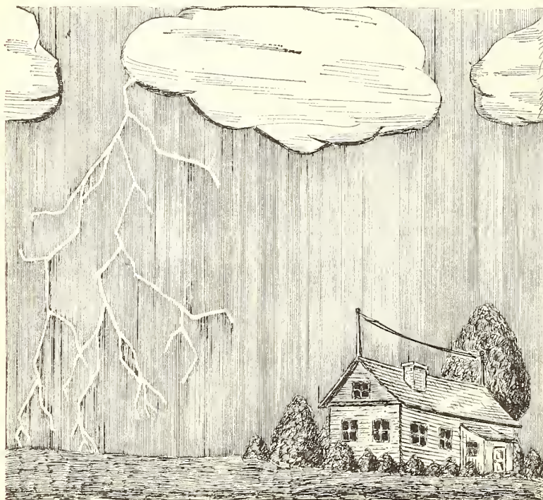
NATURAL CONDENSERS—STORM CLOUDS The lightning discharge illustrates the rupture of the dielectric
