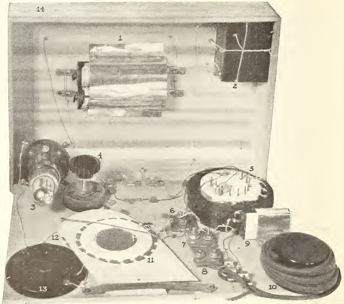
THE WORKS
