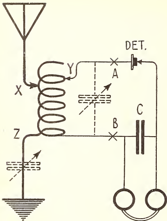
FIG. 2 An efficient and simpler circuit
