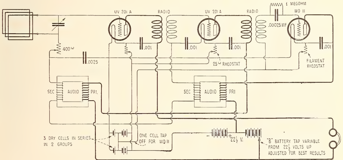
FIG. 2. THE SAME CIRCUIT ADAPTED FOR USE WITH A WD-11 OR WD-12
