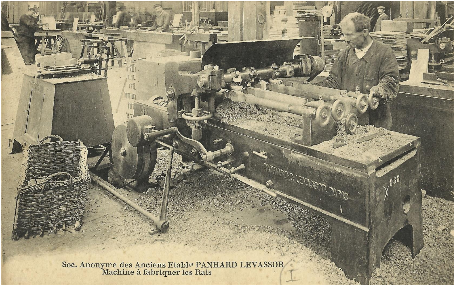
Machine for making [wheel] spokes
