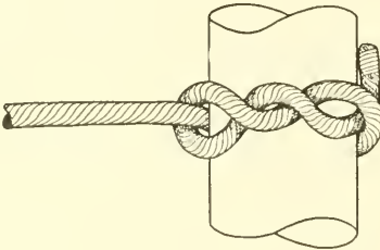
TIMBER HITCH.
