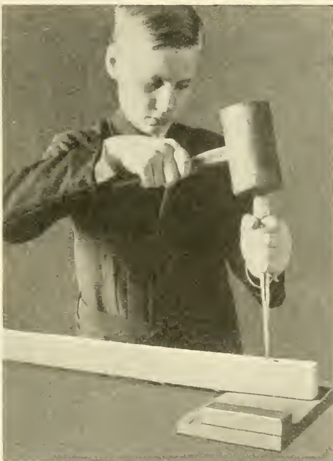
Fig. 19. Position of Chisel and Mallet for Mortising.
