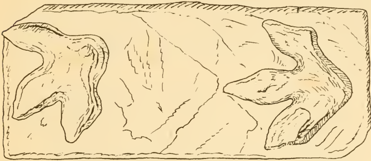
FIG. 76. Tracks of Iguanodon , much reduced. From Wealden strata, England. Modified from Hutchinson
