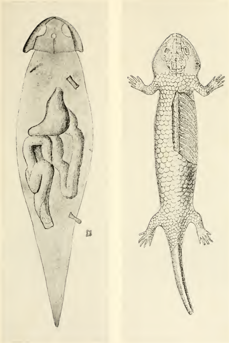
Left: The most perfectly preserved amphibian, Eumicrpeton , from Illinois. After Moodie
