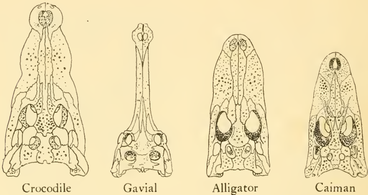
FIG. 79. Skulls of the four types of Crocodylidae viewed from above. After Charles C. Mook
