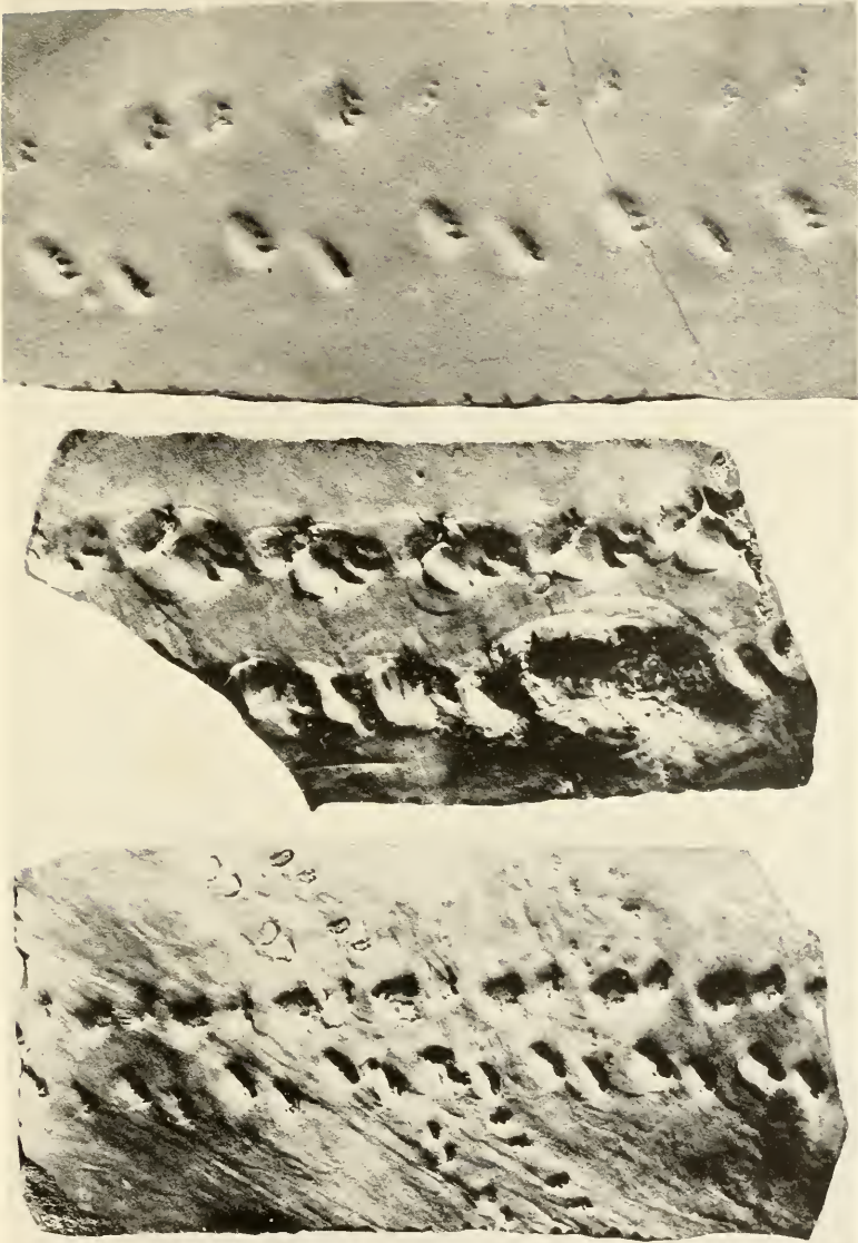
Tracks from the Coconino sandstone, Grand Canyon, Arizona. Upper, Laoporus noblei ; middle, Agostopus , with part of trail blotted out by a larger track; lower, Baropezia , crossed by Laoporus . In the National Museum
