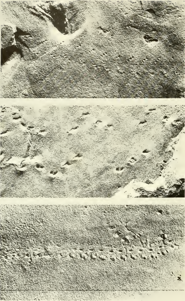
Trails of invertebrate animals from the Coconino sandstone, Grand Canyon, Arizona. In the National Museum
