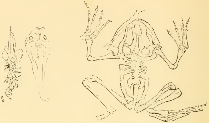
FIG. 50. Fossil larvae and fossil frog, Paleobatrachus , from the Miocene of Bohemia. After Wolterstorff and Meyer
