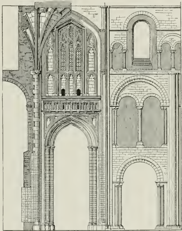
DIAGRAM SHOWING WYKEHAM'S TRANSFORMATION OF THE NAVE.
