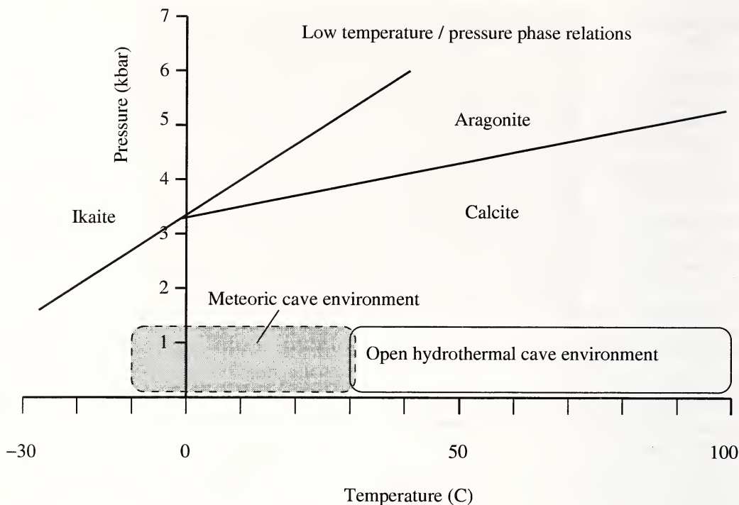
Figure 3. Stability Diagram for \text{CaCO}_3 at low temperatures and pressures shows that calcite is the expected polymorph in caves at atmospheric pressure. Based on Carlson (1983)
