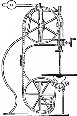
BAND SAW.
