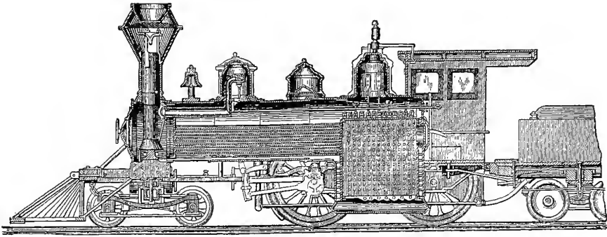
AMERICAN LOCOMOTIVE—CENTRAL LONGITUDINAL SECTION.
