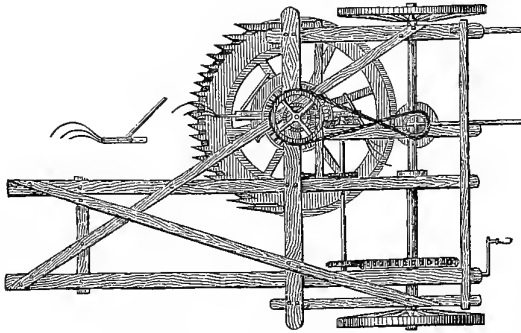
GLADSTONE'S REAPING MACHINE, ENGLAND, 1806.
