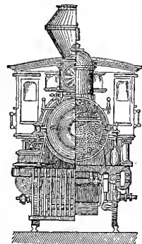
AMERICAN LOCOMOTIVE—END ELEVATION AND TRANSVERSE SECTION.
