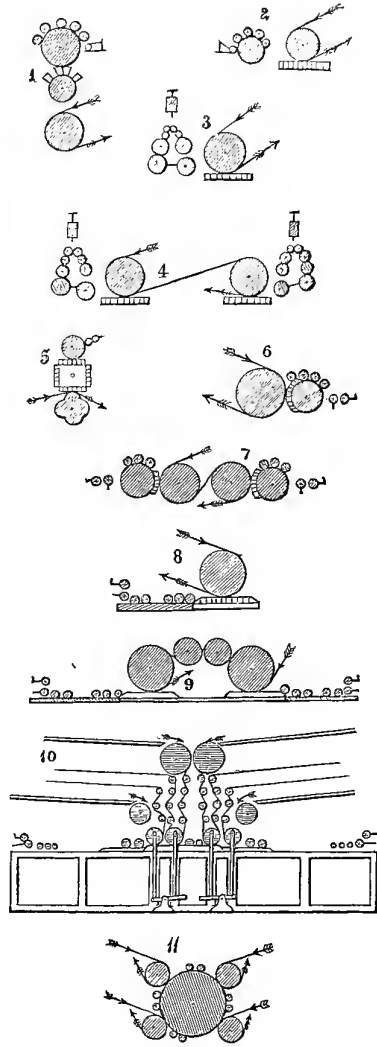
PRINCIPLES OF ACTION OF POWER-PRESSES.
