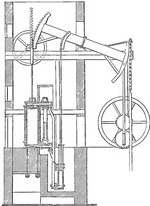
WATT'S DOUBLE-ACTING STEAM-ENGINE, 1769.
