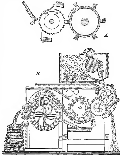
WHITNEY'S COTTON-GIN.
