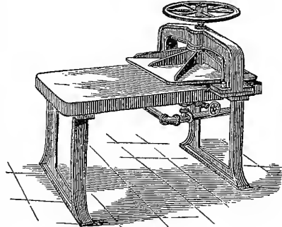
STEREOTYPE MOULD-DRYING PRESS—PAPER PROCESS.
