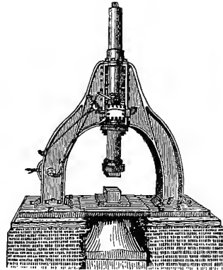
NASMYTH'S DOUBLE-FRAME STEAM-HAMMER.
