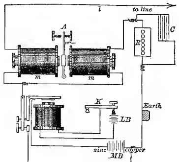
DUPLIX TELEGRAPH.
