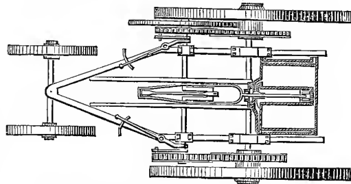
TREVETHICK AND VIVIAN'S LOCOMOTIVE, MERTHYR-TYDVIL, 1805.
