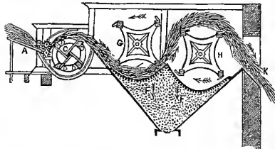
MEIKLE'S THRESHING MACHINE, 1786—INTERIOR VIEW.
