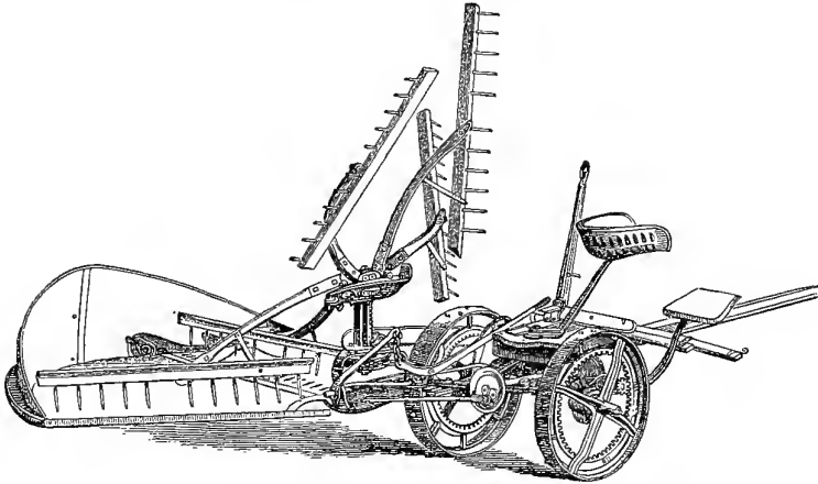
THE AMERICAN SELF-RAKING REAPING MACHINE ("CHAMPION" PATTERN).
