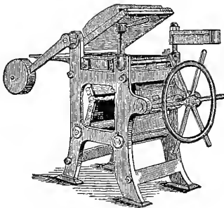
ELECTROTYPING PRESS.
