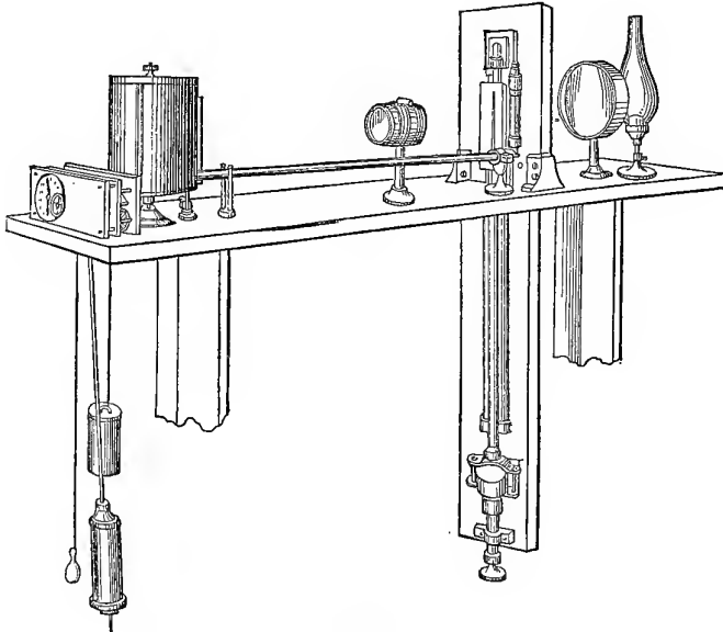
THE BAROGRAPH.
