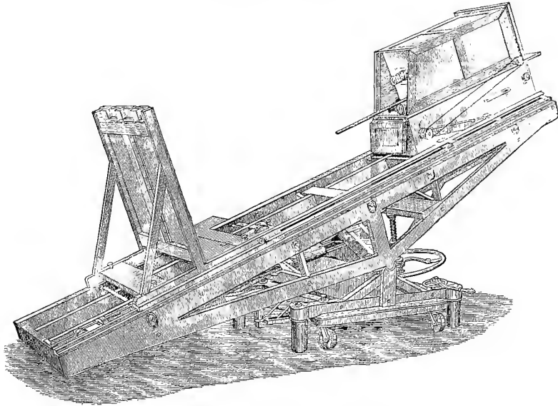
OSBORNE'S COPYING CAMERA AND TABLE.
