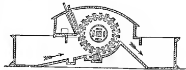
PULPING ENGINE.
