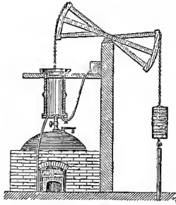
NEWCOMEN'S STEAM-ENGINE.
