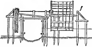
PERRONET'S CHAPELETS (CHAIN-PUMPS) AT ORLEANS, FRANCE.
