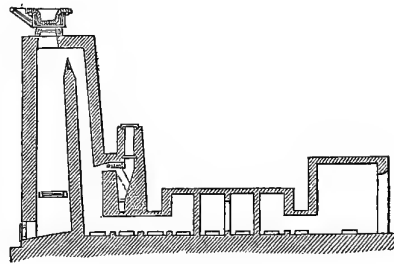
STETEFELDT'S ROASTING FURNACE.
