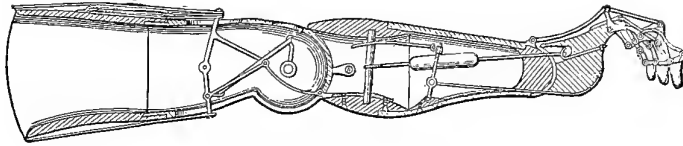
OONDELL'S ARTIFICIAL ARM. (Longitudinal section of left arm.)
