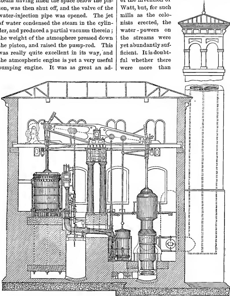
SINGLE-ACTING CORNISH PUMPING ENGINE.
