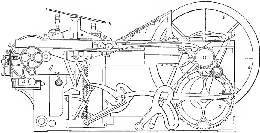
ADAMS PRESS.
