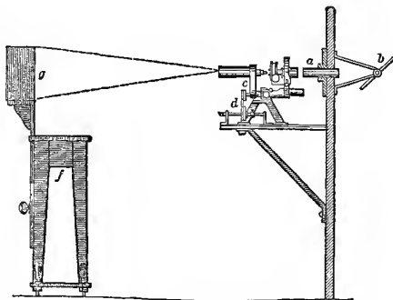
WOODWARD'S MICRO-PHOTOGRAPHIC APPARATUS (WITH SOLAR LIGHT).
