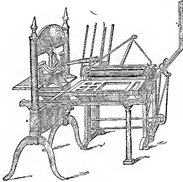
"WASHINGTON" PRESS.
