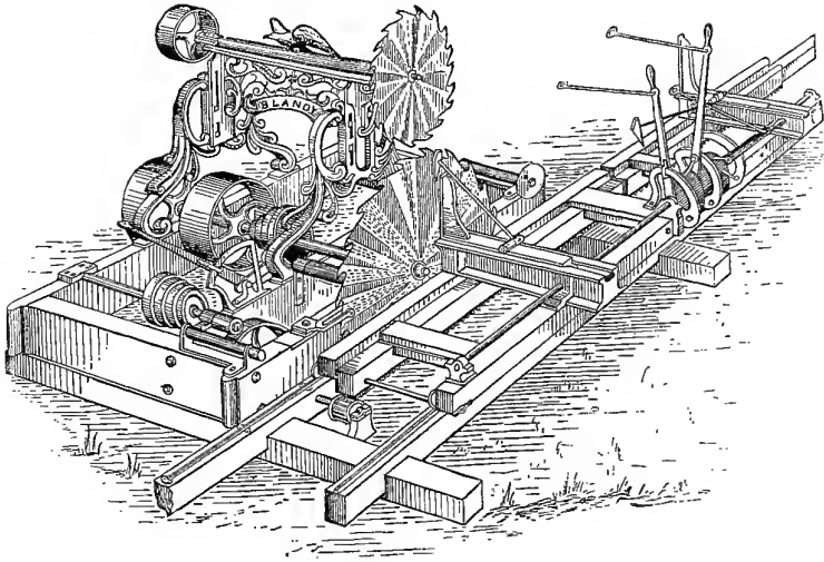
PORTABLE CIRCULAR SAW.
