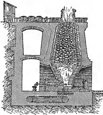
MODERN BLAST-FURNACE.
