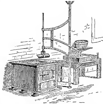
STEREOTYPE CASTING APPARATUS—PLASTER PROCESS.
