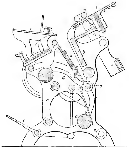
GORDON JOB PRESS.
