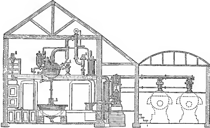
MODERN SUGAR PROCESS.
