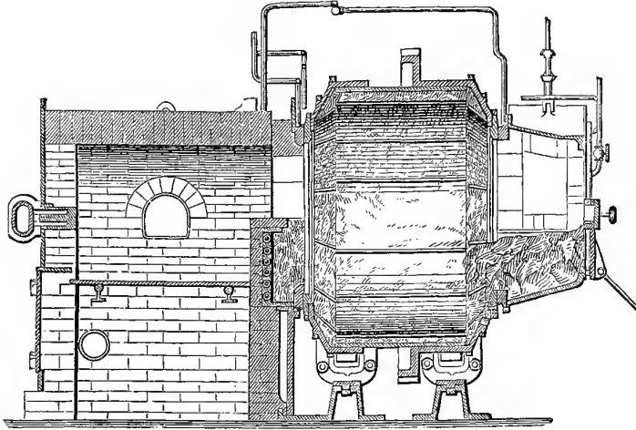
DANKS'S MECHANICAL PUDDLIER.
