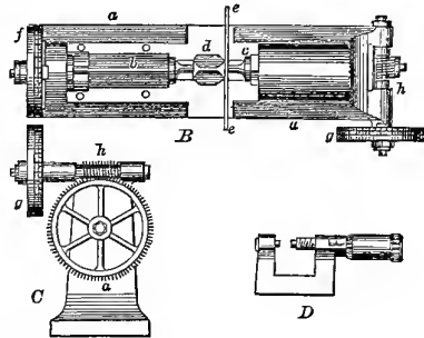
WHITWORTH'S MILLIONTH MEASURING GAUGE.
