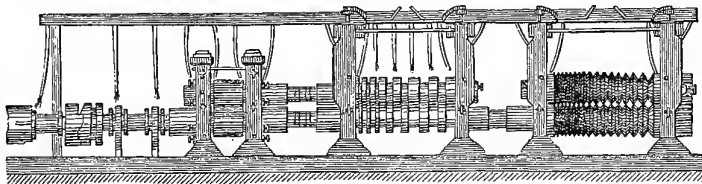
ROLLING-MILL FOR IRON BARS.
