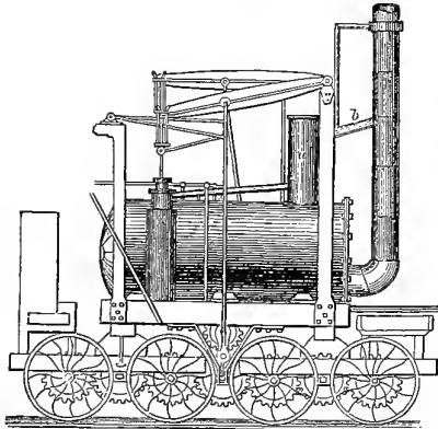
HEDLEY'S LOCOMOTIVE, "PUFFING BILLY," 1813.
