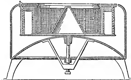
CENTRIFUGAL FILTER.
