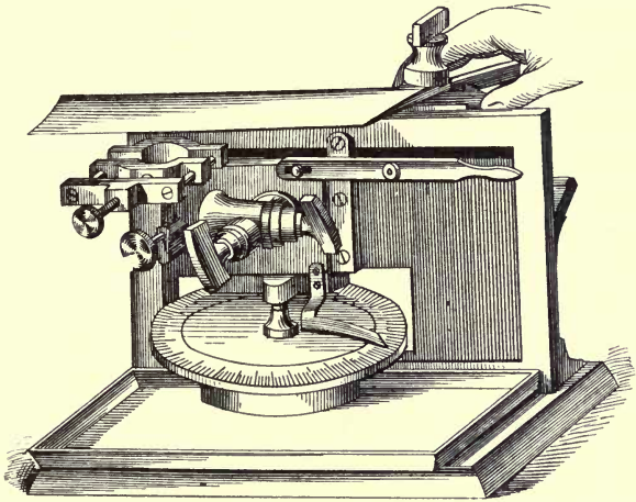
Schanze's microtome.
