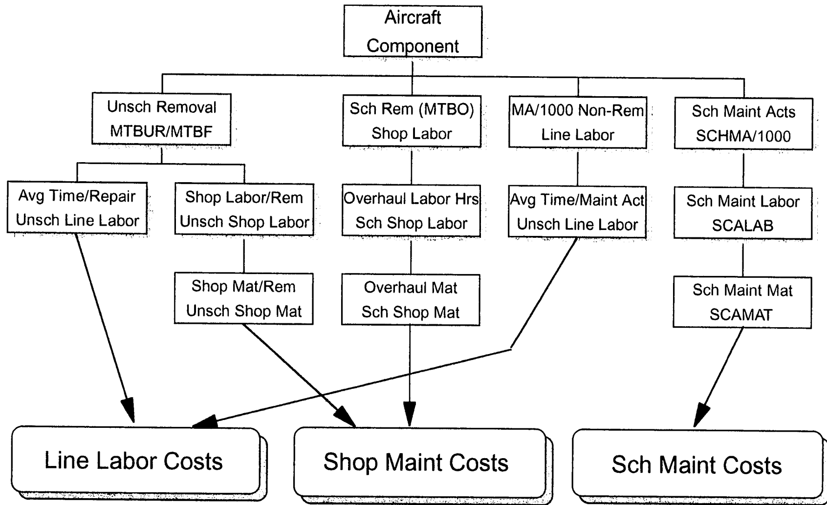
Figure 3.1 Originally Designed Structure of the DCM
