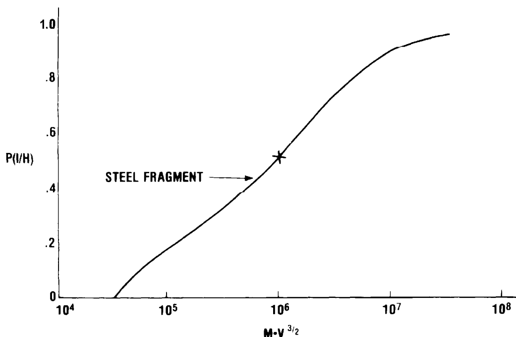
Fig. 2-1. The probability that a steel fragment will incapacitate a soldier. P(I/H) represents the probability of incapacitation if the soldier is wounded; M , the fragment's mass in grains; and V , its velocity in fps. Notice that the relationship is semilogarithmic: The point labelled X can be interpreted to mean that an irregular steel fragment with mass and velocity such that M \times V^{3/2} = 1 \times 10^6 striking a soldier at random will prevent him from performing 50% of his duties in an assault that began 5 minutes after he was wounded.
