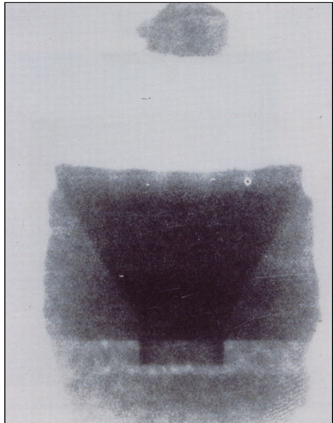
Fig. 1-50. The dual-purpose submunition shown in this roentgenogram measures about 4 cm in diameter and 8 cm in length. It contains about 30 g of explosive. The characteristic funnel shape of the shaped-charge warhead can be clearly seen. It not only can penetrate 80 mm of armor, but also can generate many antipersonnel fragments.
