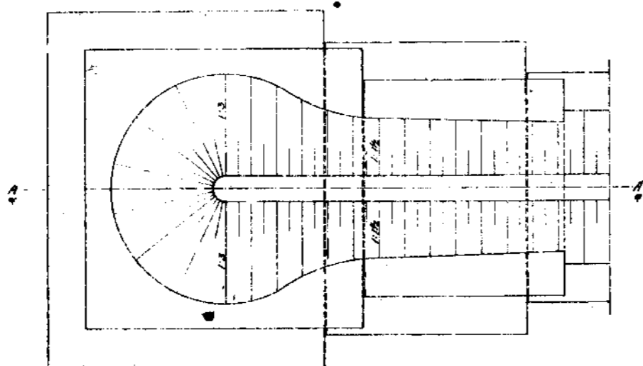
丙式堤工端部平面圖 Head of cribwork Type C.
