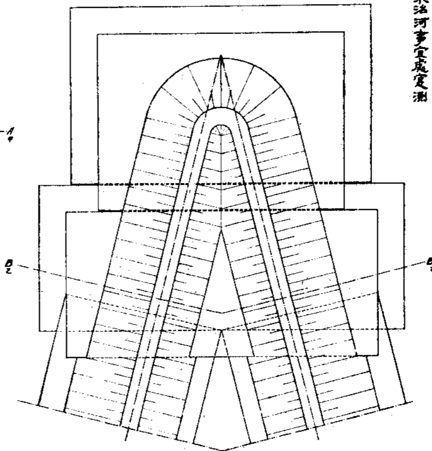
Trainingwork Type D 丁式堤工
