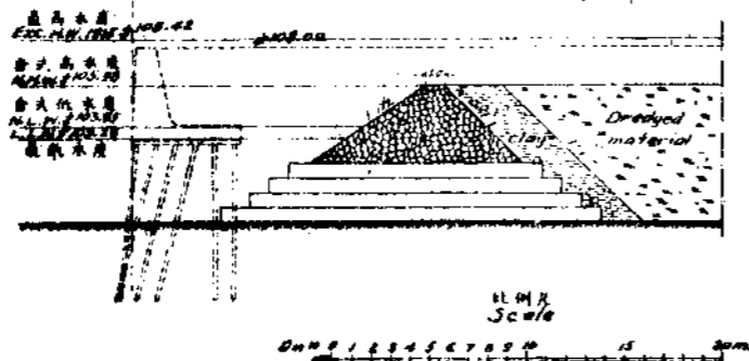
戊式填土埝堤剖面圖 Cross-section of reclamation wall Type E.
