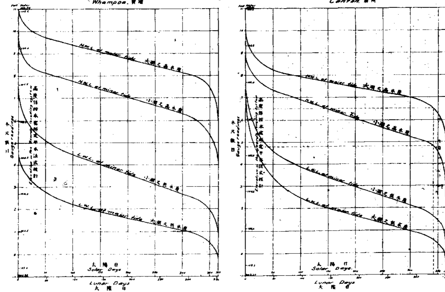
Curves showing frequency of high and low waters, of Whampoa and Canton. Mean of the years 1913 and 1914.
