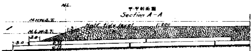
戊式填土埝堤剖面圖 Cross-section of reclamation wall Type E.
