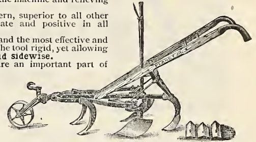
No. 9 Horse Hoe and Cultivator.
