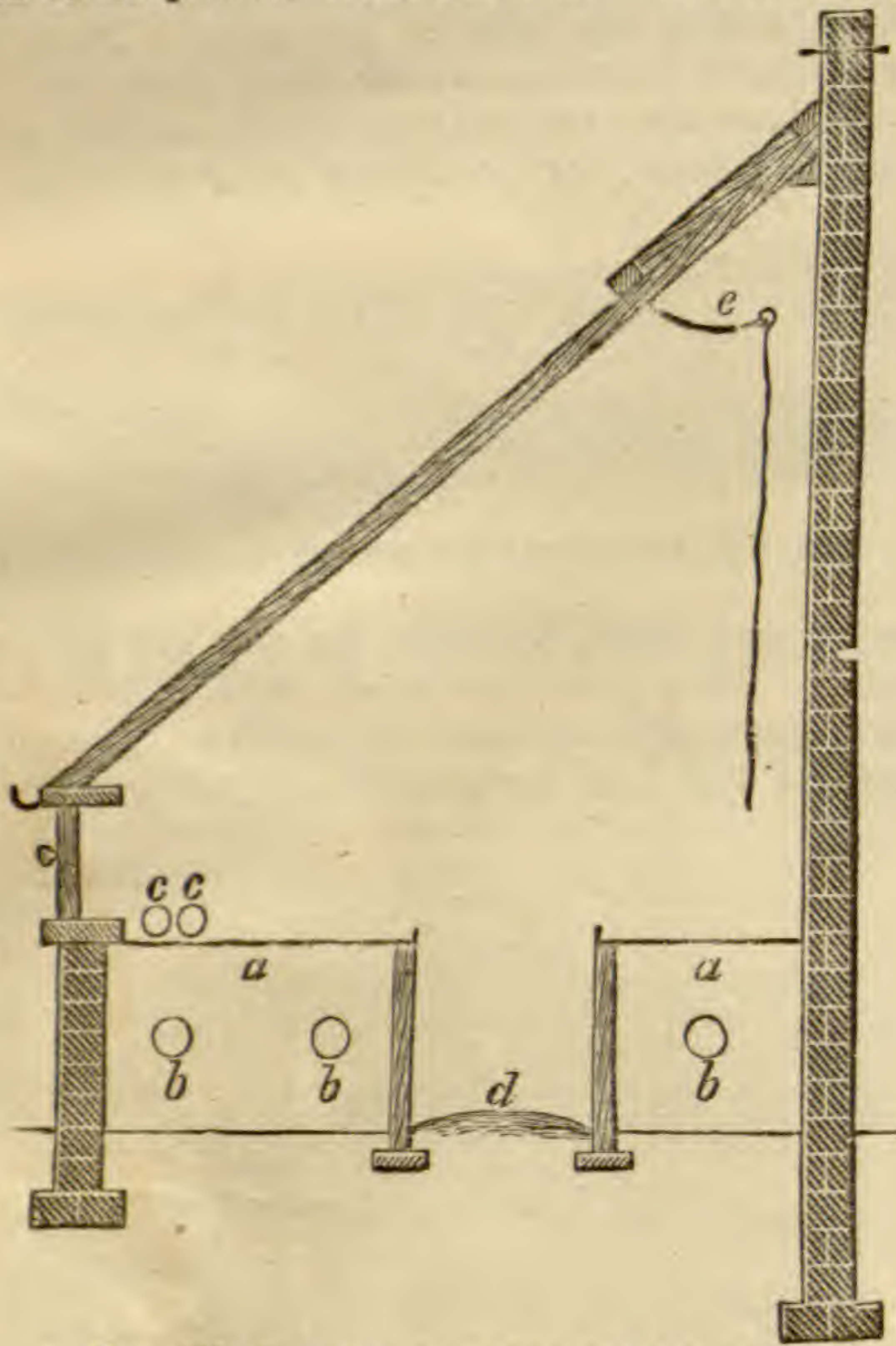
FIG. 561. SECTION OF LEAN-TO HOUSE.
