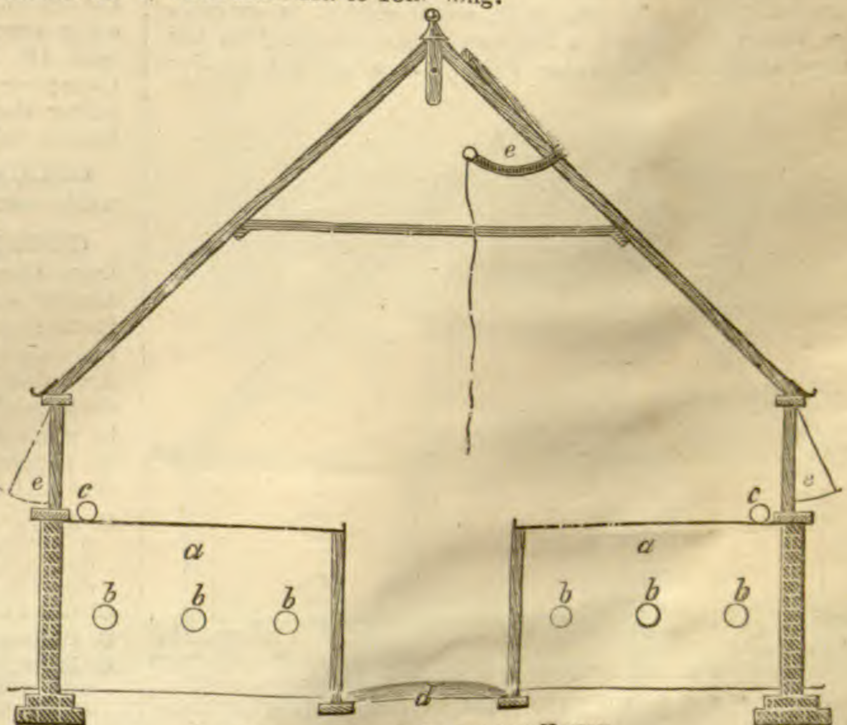
FIG. 560. SECTION OF SPAN-ROOF HOUSE a a , Space for Bottom Heat; b b b b b b , Hot-water Pipes; c c , Pipes for Top Heat; d , Path; e e e , Ventilators.
