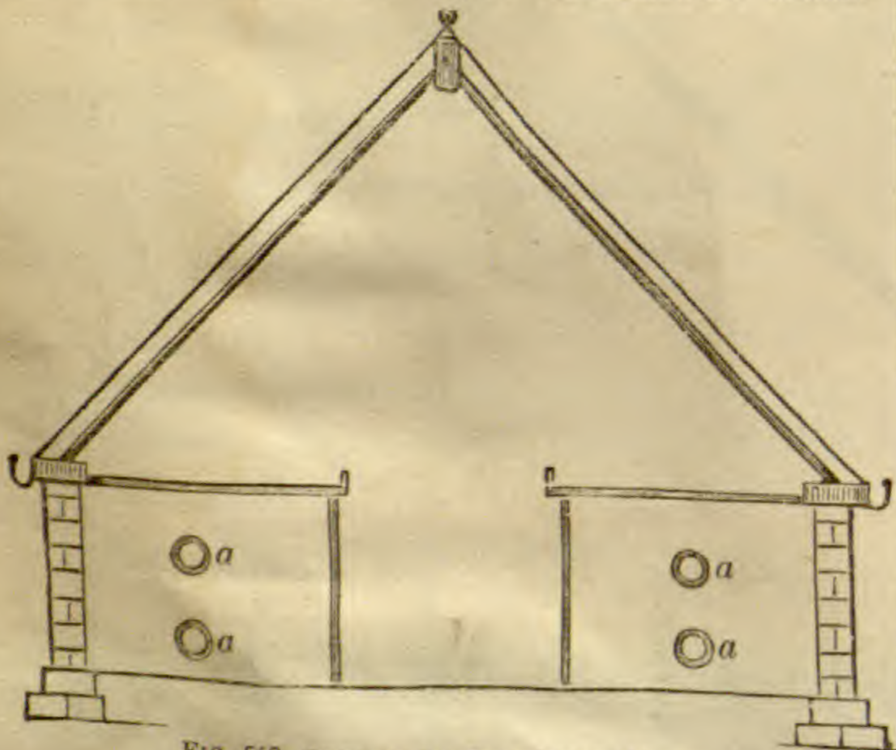
FIG. 562. SECTION OF SPAN-ROOF HOUSE.
