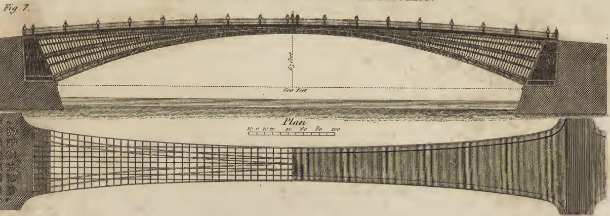
BRIDGE PROPOSED BY MESS: TELFORD AND DOUGLASS.
