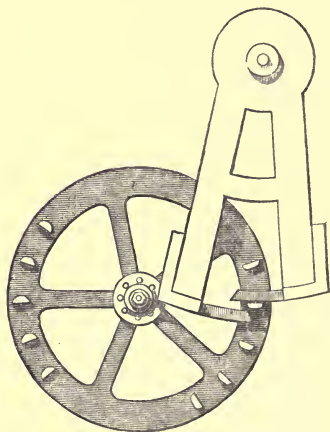
French Single-Pin Escapement.
