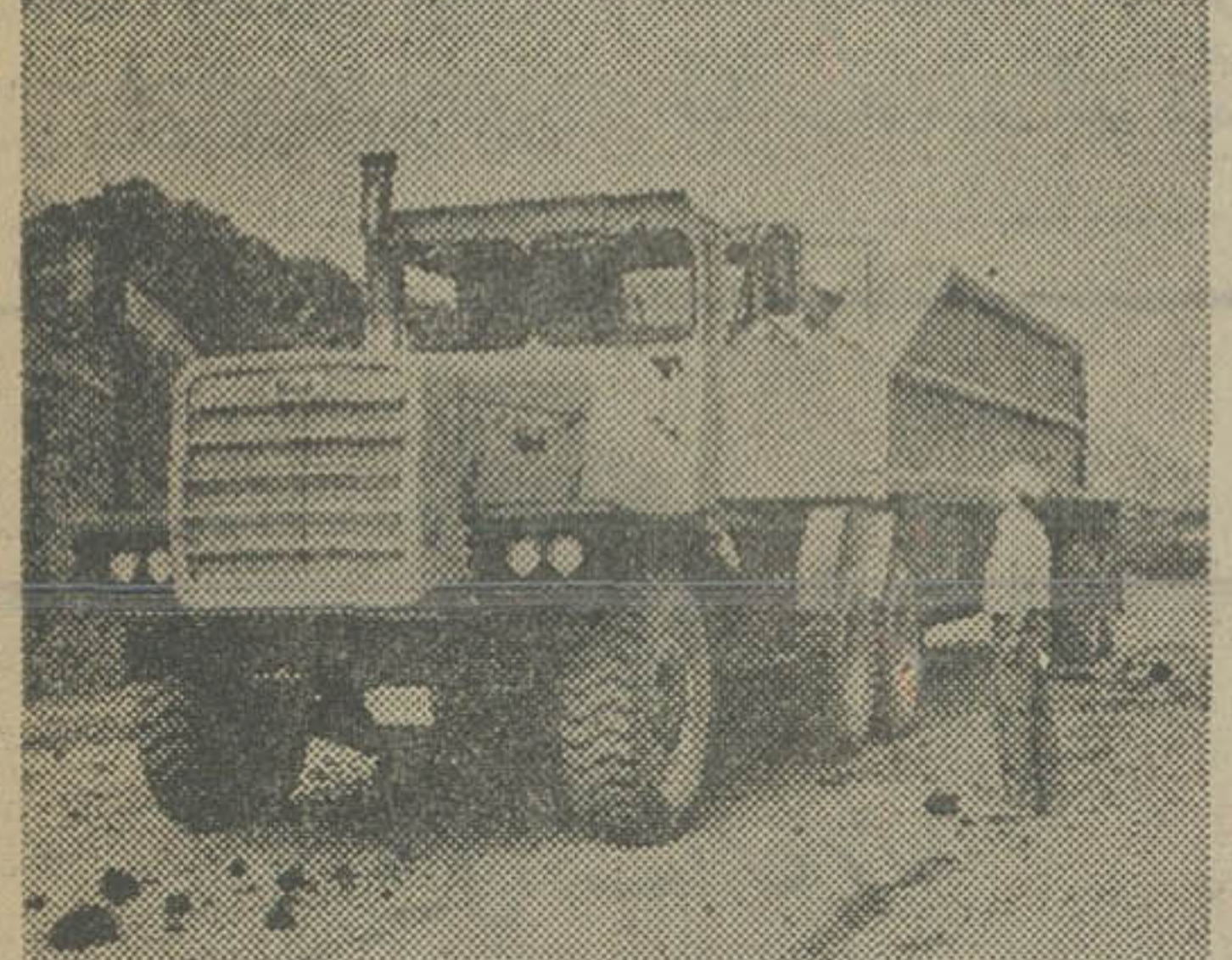
120-TON TRACTOR-BOTTOM DUMP SEMI-TRAILER
