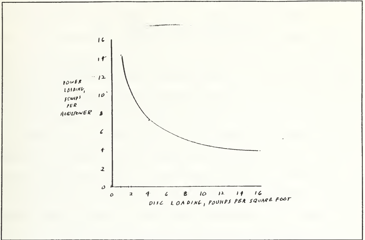
Figure 11 Rotor Performance for Design Conditions
