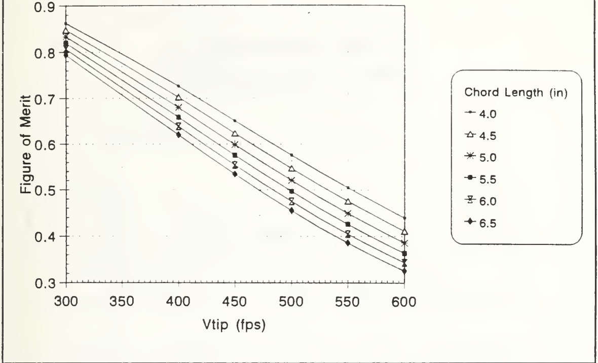
Figure 15 Figure of Merit vs Blade Tip Speed
