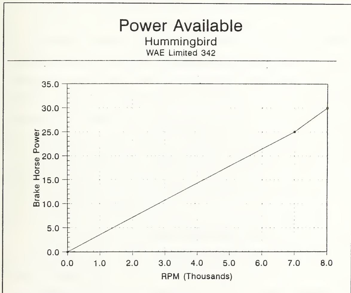
Figure 32 Power Available vs RPM
