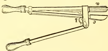
FIG. 150.—Foote's stock splitter.
