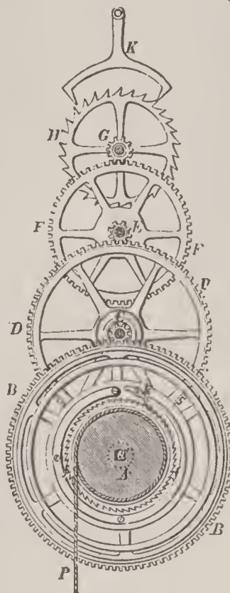
Clock-work.
