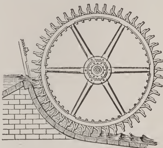
Breast-wheel.
