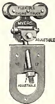
No. 12. Giant New Way Hanger. $2.40 per pair Giant New Way Track. 21c per foot Intermediate Brackets. 15c each End Brackets. 15c each
