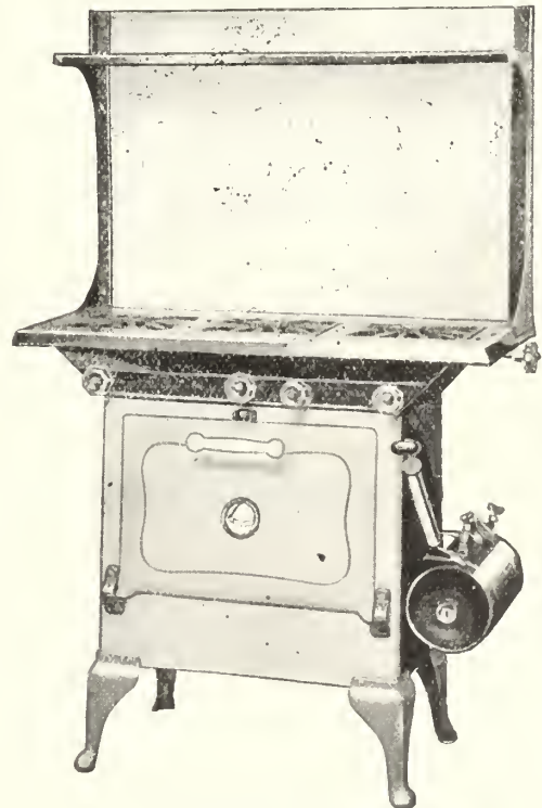
No. 3031. Low Oven Rangette with No. 3 Hi-shelf
