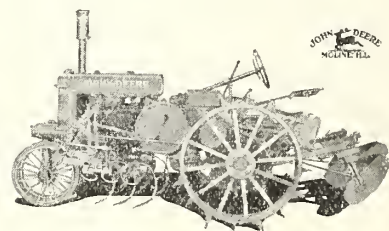
GP-443 Two-Row Cultivator—Spring Tooth, with No. GP-5 Two-Row Potato Hoe
