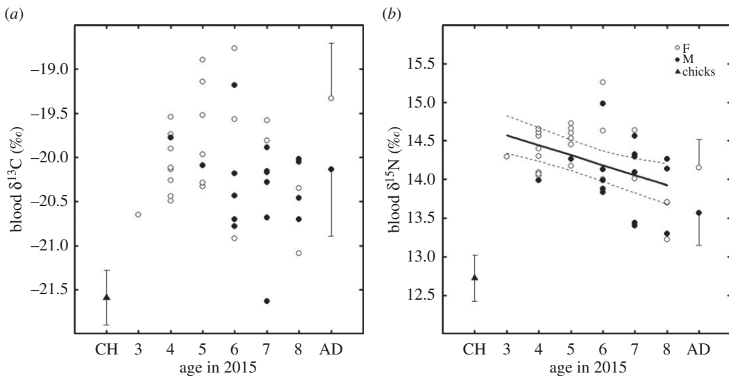
Figure 2. Age-related changes in blood (a) \delta^{13}C and (b) \delta^{15}N values in immature wandering albatross from Crozet Islands. Mean \pm s.d. is also presented for chicks (CH, authors' unpublished data 2007) and adults (AD, young breeders) [8].
