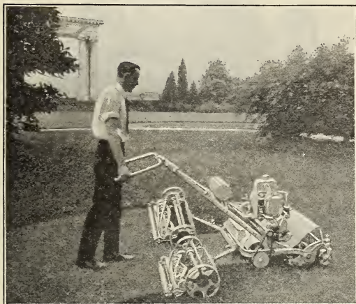
MODEL "L" WITH GANG UNITS ATTACHED
