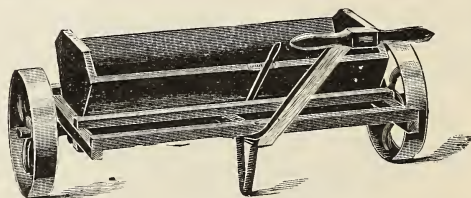
FERTILIZER SOWER, THE STEVENS' HAND
