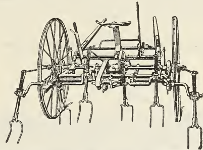
HAY TEDDER, McCORMICK-DEERING
