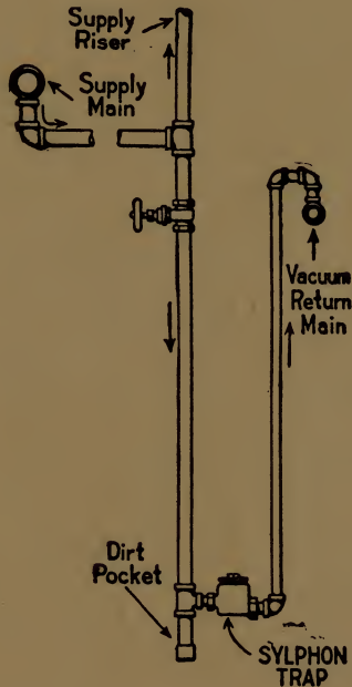
Fig. 109.—Method of dripping supply risers through Webster Siphon Trap into vacuum return line.
