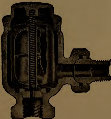
Fig. 113.—Webster Water-Seal Trap.
