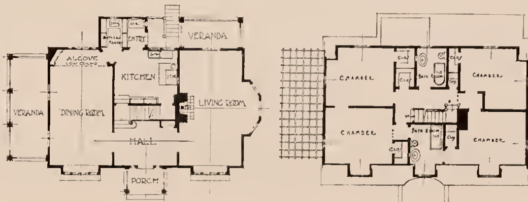
Floor plans of a house that can be furnished for $1,500
