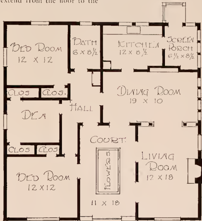
Floor plan
