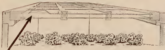
The principle—Two layers of glass with a \frac{1}{8} -inch layer of dry still air
