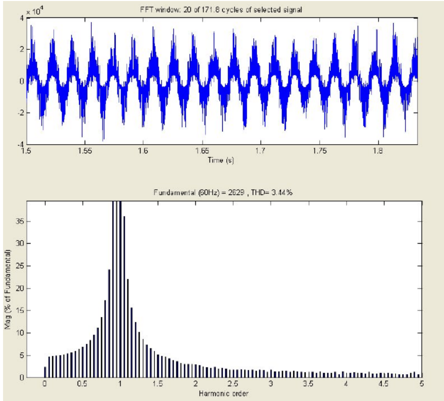
Figure 44: Simulation 9 Voltage Waveform and FFT
