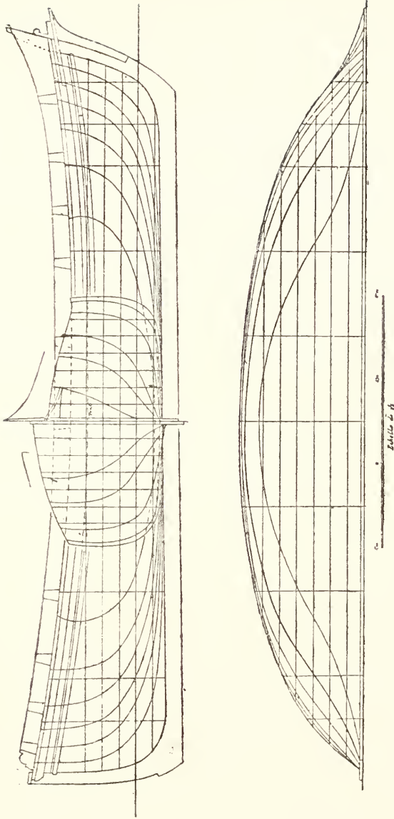
FIG. 130.—LINES OF MARSEILLES PILOT-BOAT. (See p. 329.)
