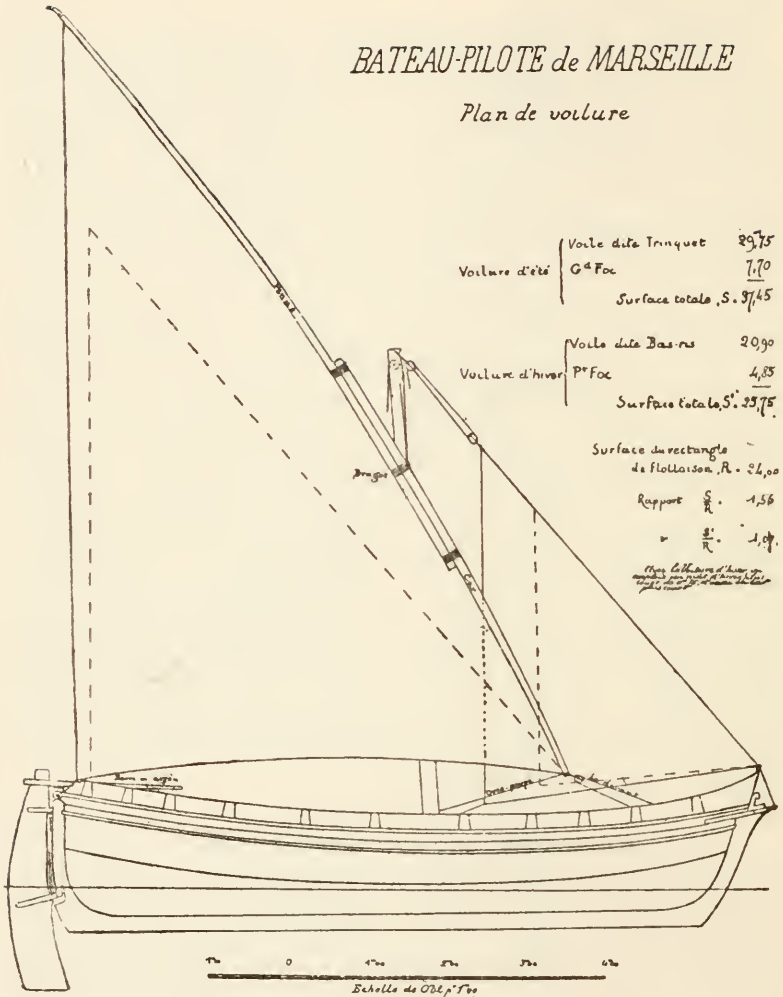
FIG. 129.—SAIL-PLAN OF MARSEILLES PILOT-BOAT.
