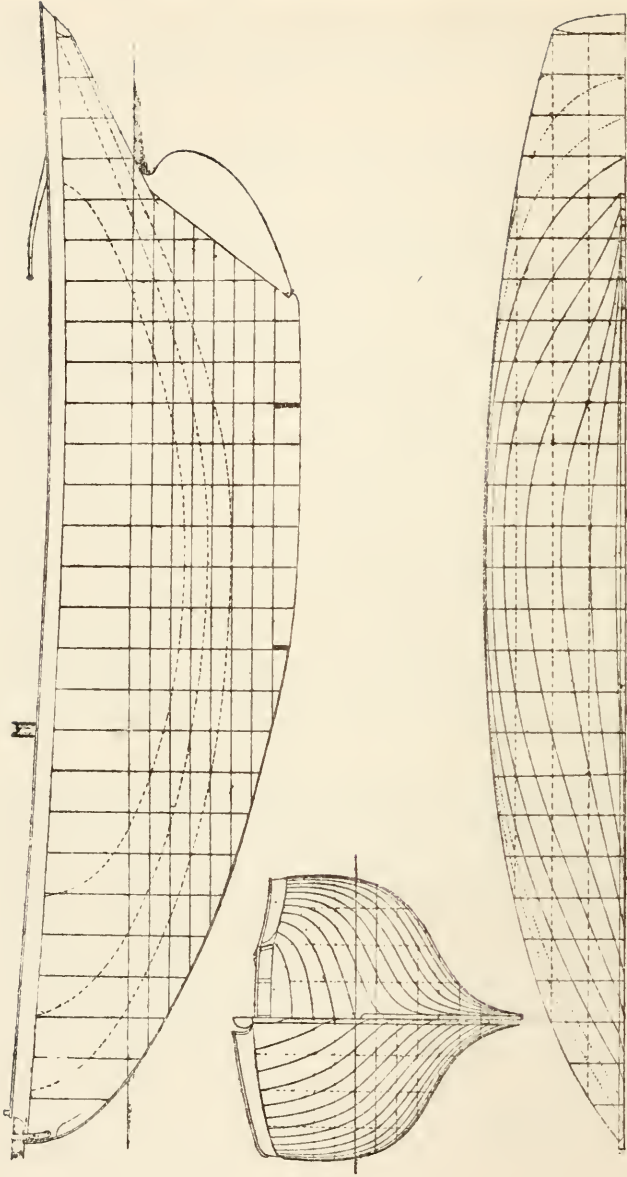
FIG. 66.—LINES OF BRISTOL CHANNEL PILOT-CUTTER "FAITH."
