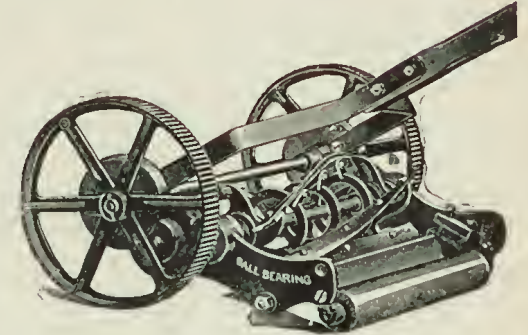
Elliott's Victory Ball-Bearing Lawn Mower
