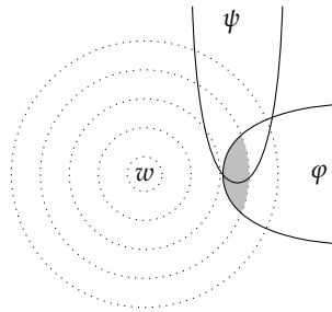
Figure 60.4: False counterfactual, false opposite
