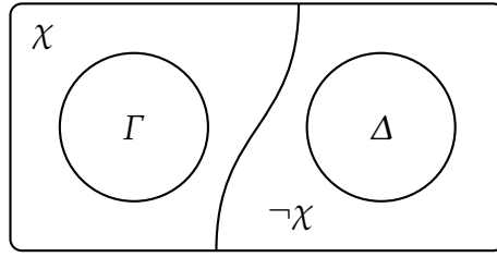
Figure 27.1: \chi separates \Gamma and \Delta
