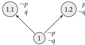
Figure 54.1: A countermodel to \Box(p \vee q) \rightarrow (\Box p \vee \Box q) .
