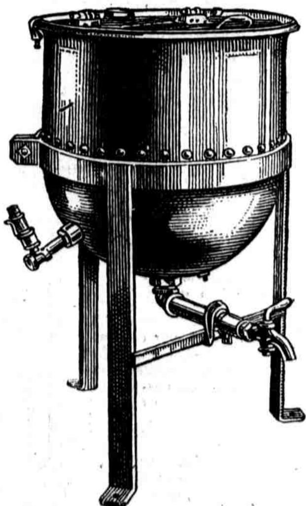
"Wear-Ever" Steam Jacketed Kettle
