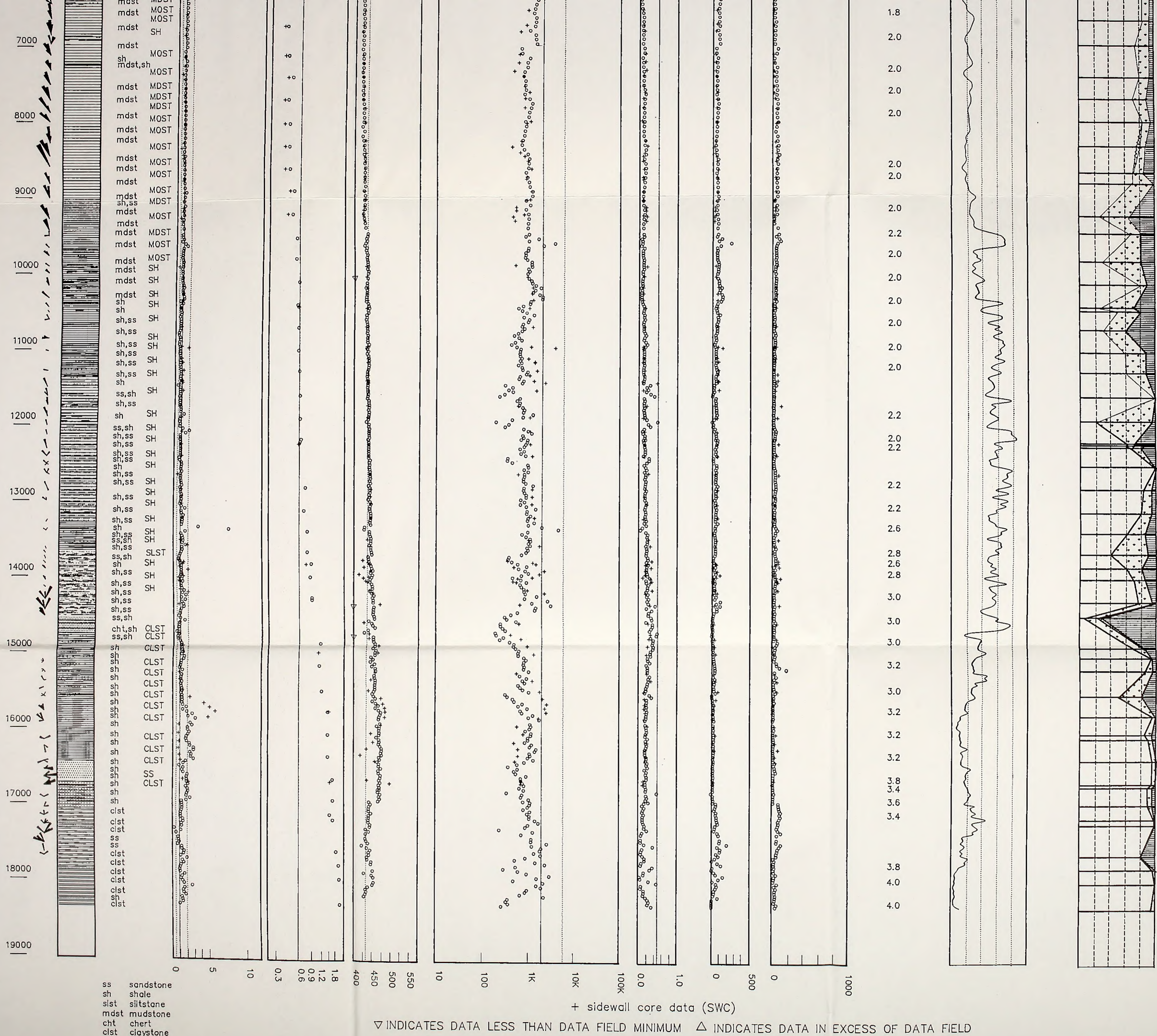
PLATE 3. GEOCHEMICAL DATA
