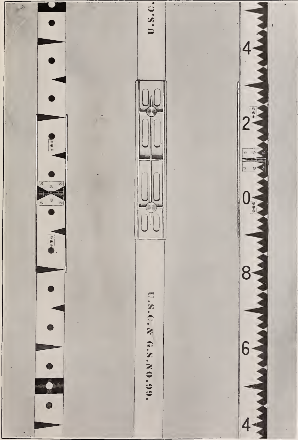
STADIA RODS.
