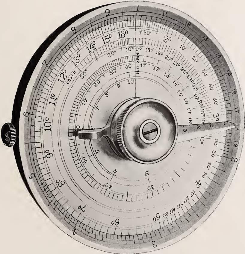
HYP SOGRAPH.
