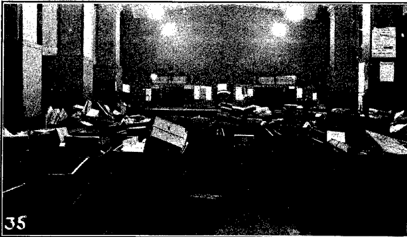
Fig. 17.—Parcel post tables and racks illuminated by unit No. 3 with a 300-watt lamp, the illumination on the working plane being 6.0 foot-candles
