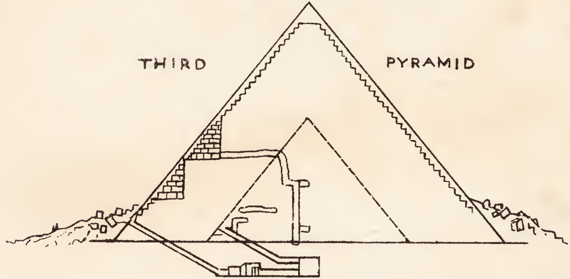
SECTIONS FROM NORTH TO SOUTH
