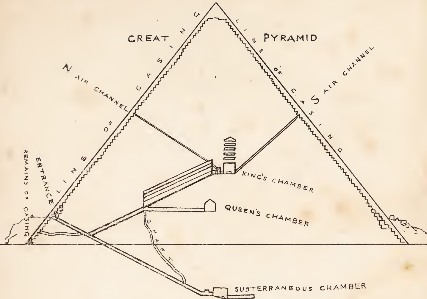
SECTIONS FROM NORTH TO SOUTH
