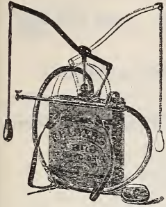
Fig. 547. Myers Knapsack Spray Pump
